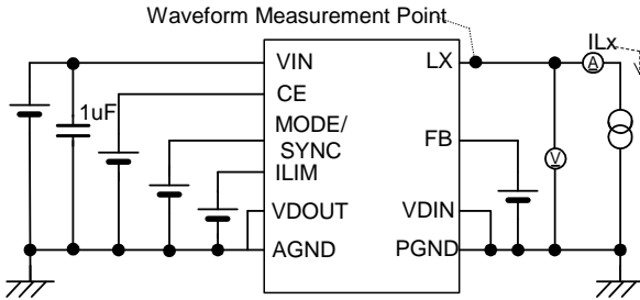
Circuit ①
