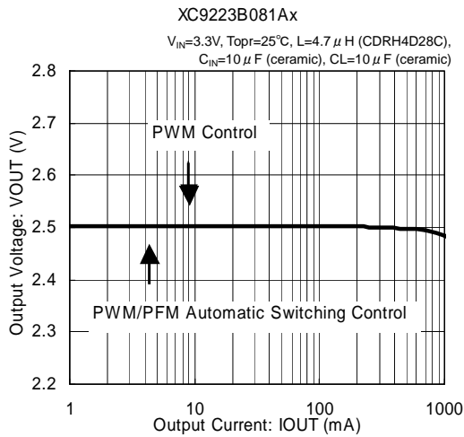
(2) Output Voltage vs. Output Current (Continued)
