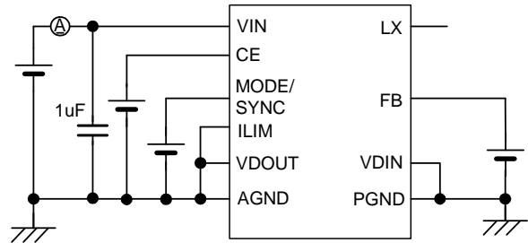
Circuit ②
