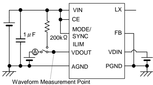
Circuit ⑦
