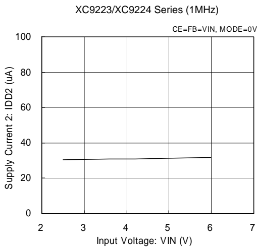
(5) Supply Current 2 vs. Input Voltage
