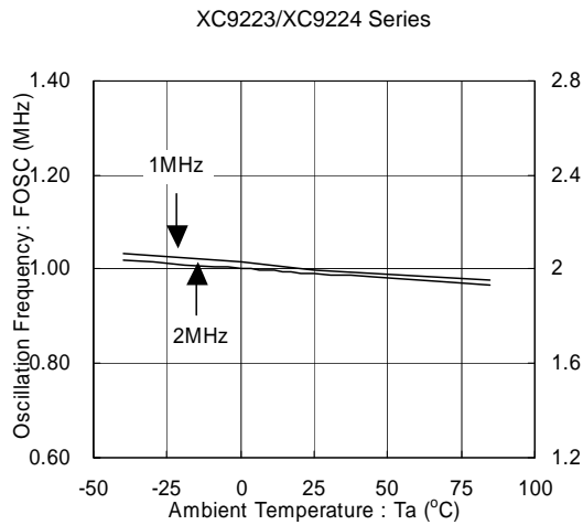
(3) Oscillation Frequency vs. Ambient Temperature
