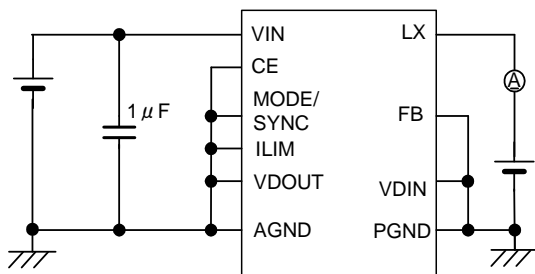
Circuit ⑥
