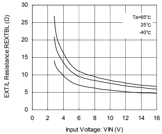
(11) EXT L ON Resistance Characteristics XC9220/21 Series
