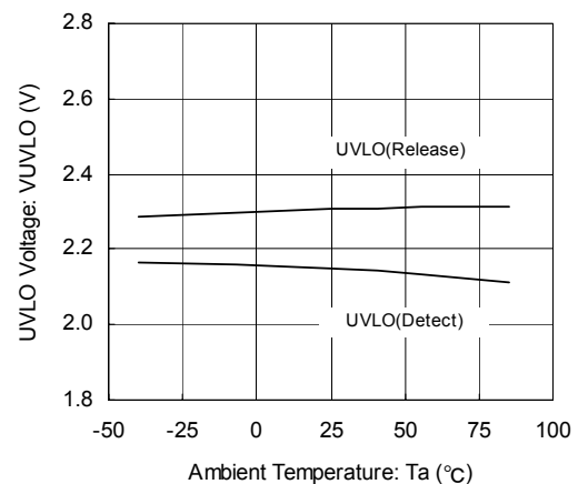
(9) U.V.L.O. Temperature Characteristics XC9220/21Series
