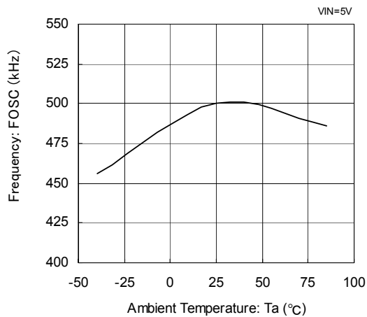
(8) Oscillation Frequency Temperature Characteristics XC9220/21x095xx
