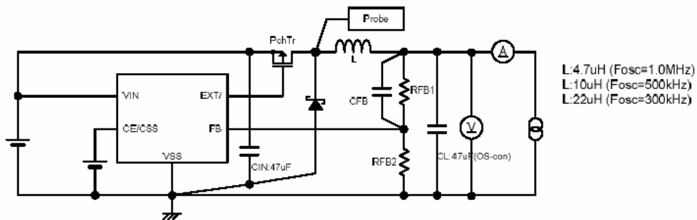
Circuit 3: Oscillation Frequency, PFMDUTY, U.V.L.O., Efficiency
