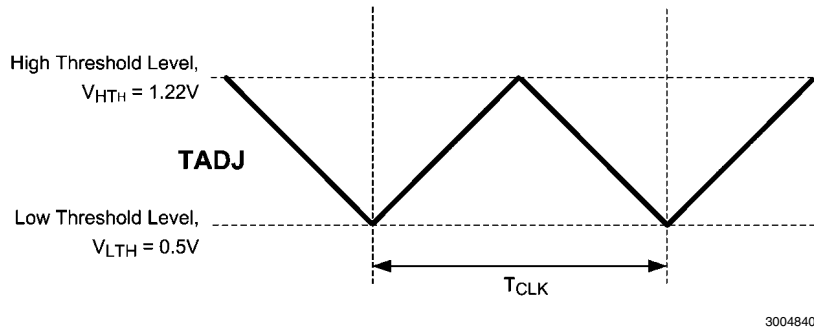
FIGURE 1. TADJ Pin Timing Waveform
