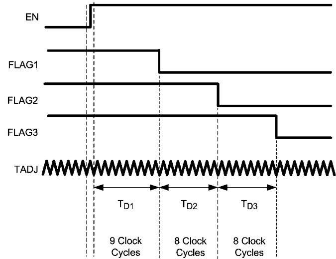
FIGURE 3. Power Up Sequence, INV High
