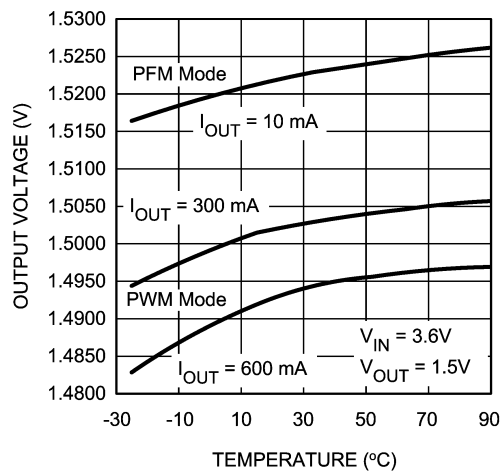
Output Voltage vs. Temperature ( V_{OUT} = 1.5V )
