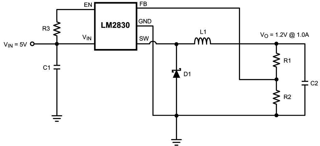
FIGURE 6. LM2830X (1.6MHz): V_{in} = 5V , V_o = 1.2V @ 1.0A
