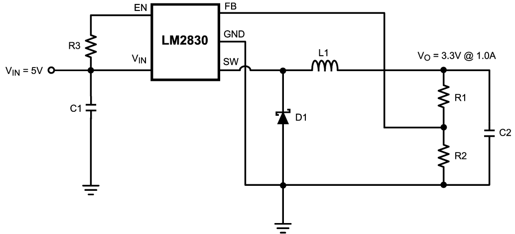
FIGURE 8. LM2830X (1.6MHz): V_{in} = 5V , V_o = 3.3V @ 1.0A
