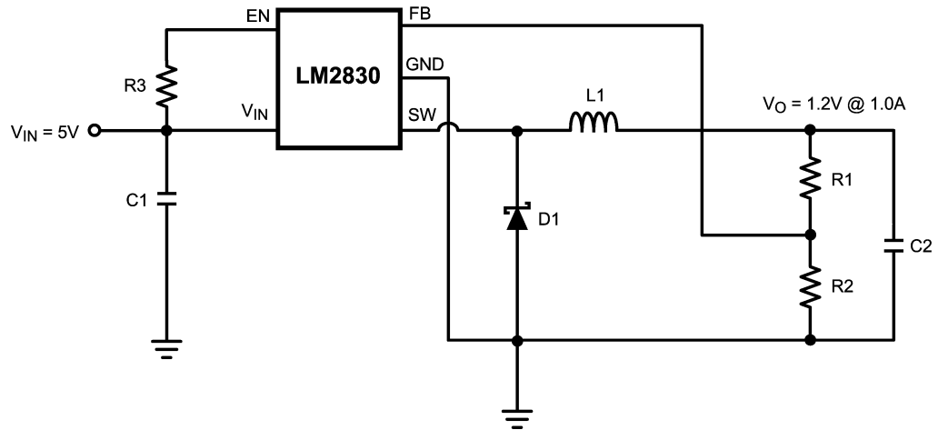
FIGURE 10. LM2830Z (3MHz): V_{in} = 5V , V_o = 1.2V @ 1.0A
