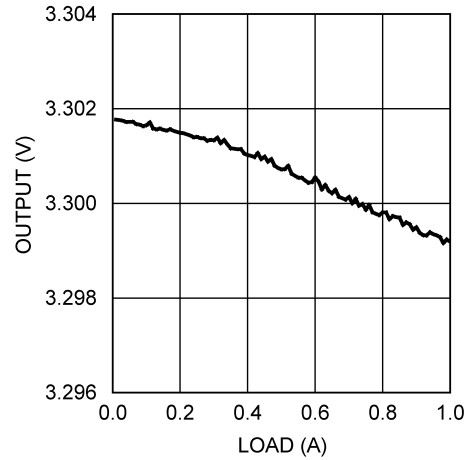
Load Regulation V_{in} = 5V, V_o = 3.3V (All Options)
