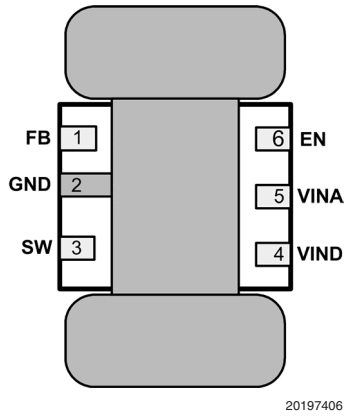
FIGURE 5. 6-Lead LLP PCB Dog Bone Layout
