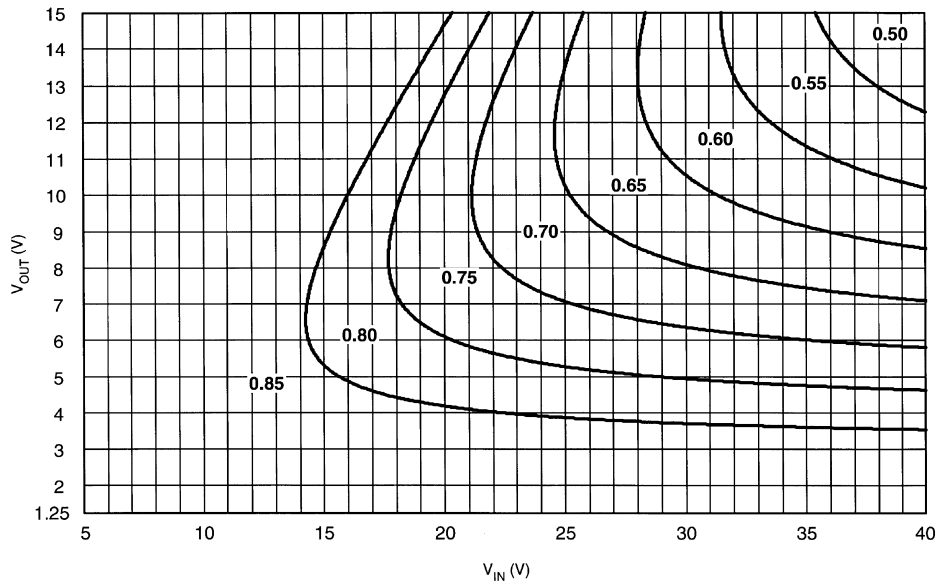
FIGURE 6. LM2825 Output Current Derating for T_J = -40^\circ\text{C} to -25^\circ\text{C}
