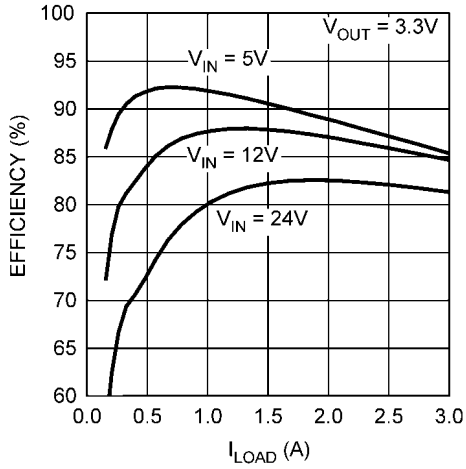
Efficiency vs. Load Current f_{SW} = 750 \text{ kHz}
