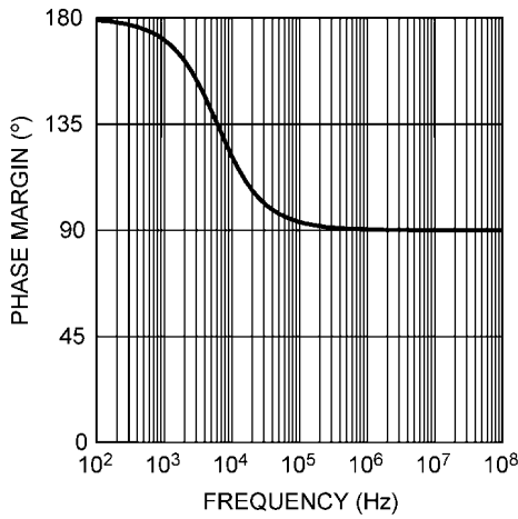
Error Amplifier Phase
