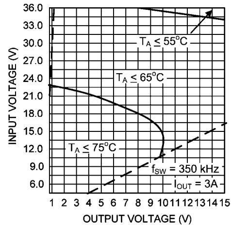
FIGURE 8. Safe Thermal Operating Areas ( I_{OUT} = 3A , f_{SW} = 350kHz )
