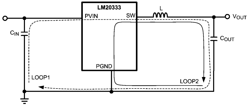
FIGURE 13. Schematic of LM20333 Highlighting Layout Sensitive Nodes
