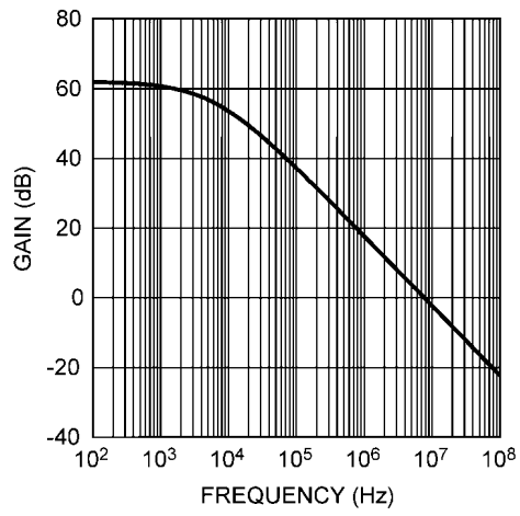
Error Amplifier Gain
