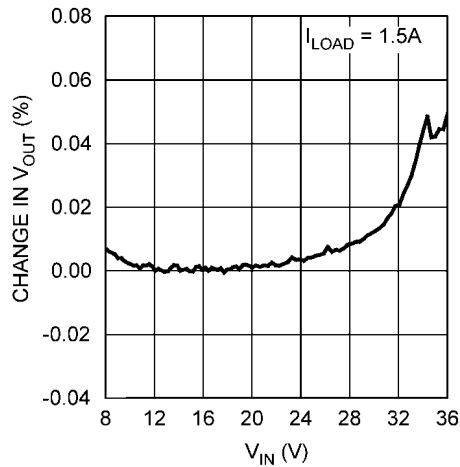
Line Regulation
