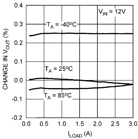
Load Regulation
