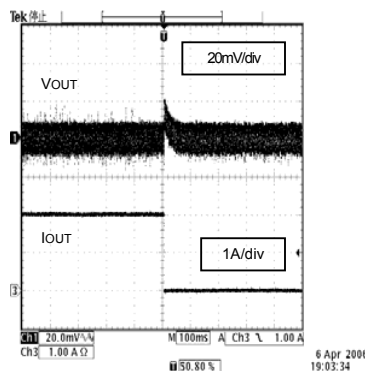
Fig.11 Load response 1
