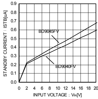
Fig.4 Standby current
