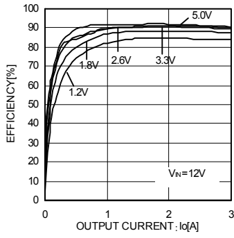
Fig.1 Efficiency 1
