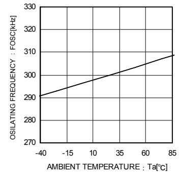
Fig.6 Frequency temperature characteristic
