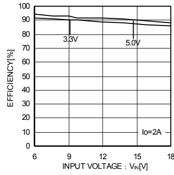
Fig.2 Efficiency 2
