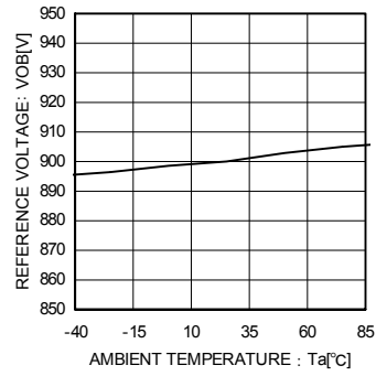
Fig.5 Standard voltage temperature characteristic
