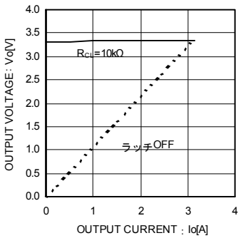
Fig.8 Loading regulation
