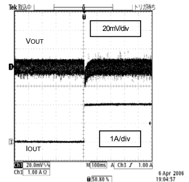
Fig.12 Load response 2
