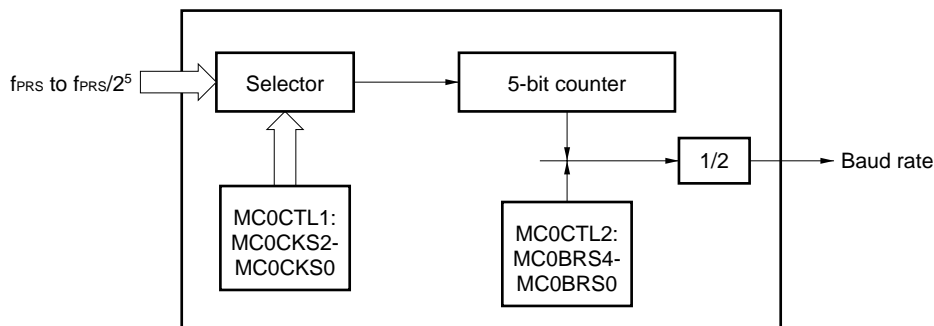
Figure 16-2. Block Diagram of Baud Rate Generator
