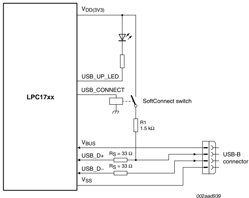
Fig 22. LPC1758/56/54/52/51 USB interface on a self-powered device
