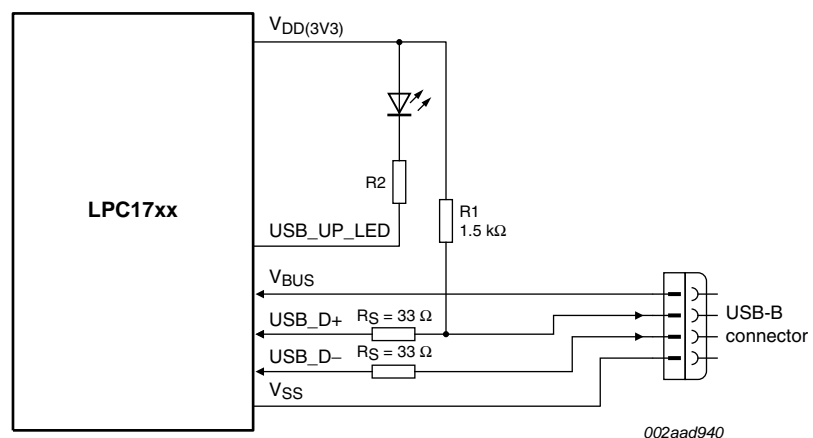
Fig 23. LPC1758/56/54/52/51 USB interface on a bus-powered device
