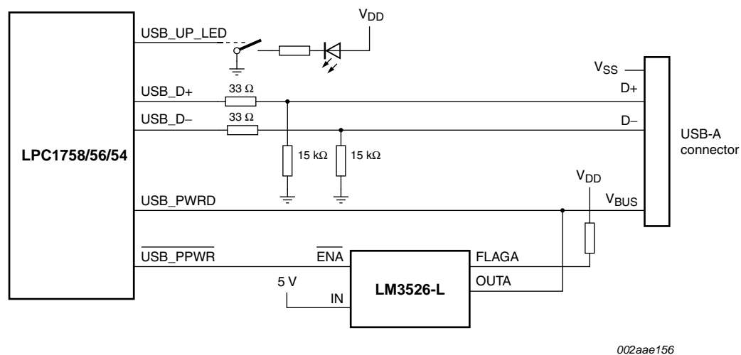
Fig 25. LPC1758/56/54 USB host port configuration
