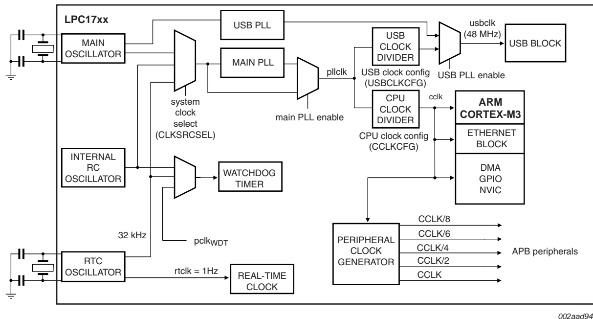
Fig 4. LPC1758/56/54/52/51 clocking generation block diagram
