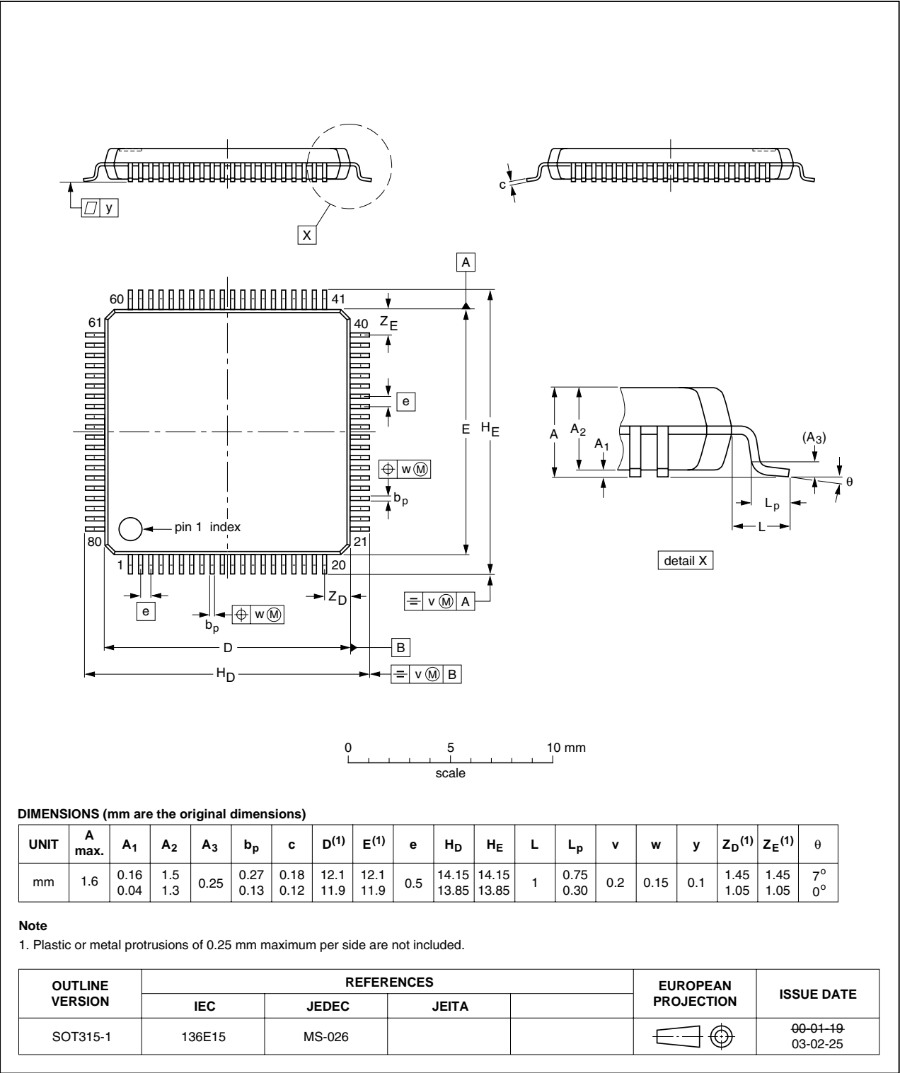
Fig 28. Package outline (LQFP80)
