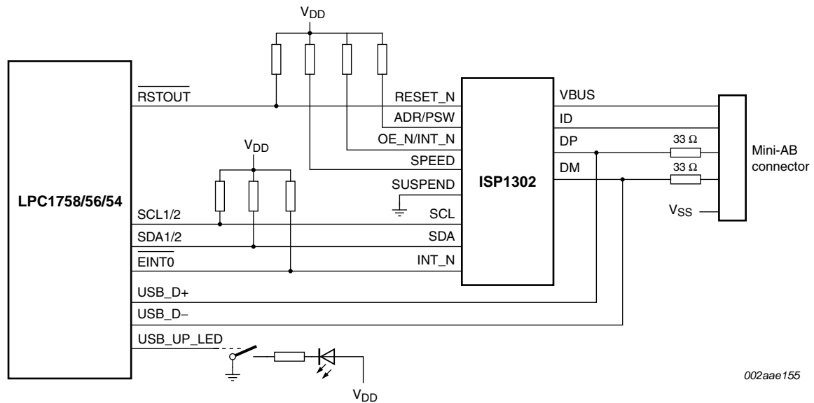
Fig 24. LPC1758/56/54 USB OTG port configuration
