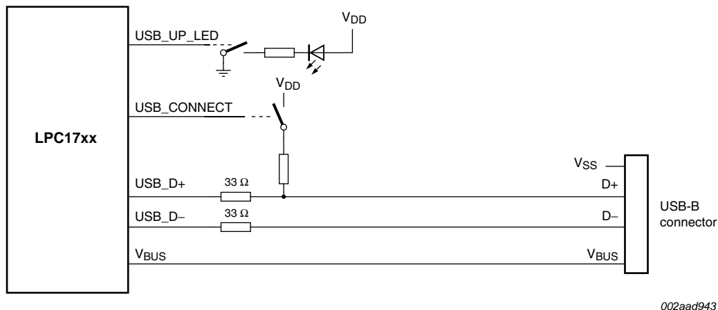
Fig 26. LPC1758/56/54/52/51 USB device port configuration
