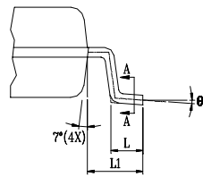
DETAIL "A" (2:1)
