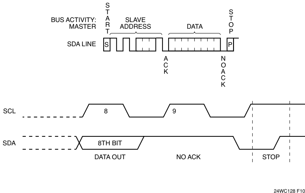
Figure 8. Immediate Address Read Timing
