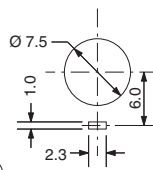
PANEL CUT-OUT
