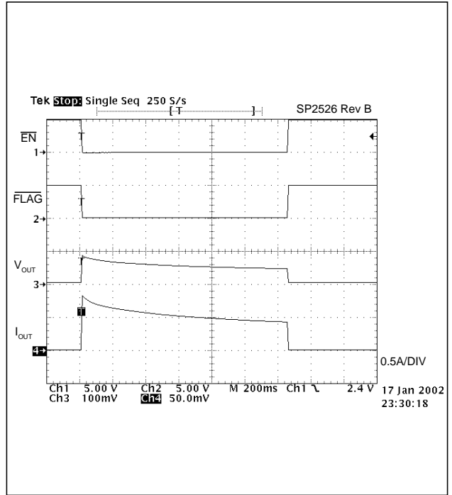
Figure 21. Short Circuit Response (Enable into Short Circuit)
