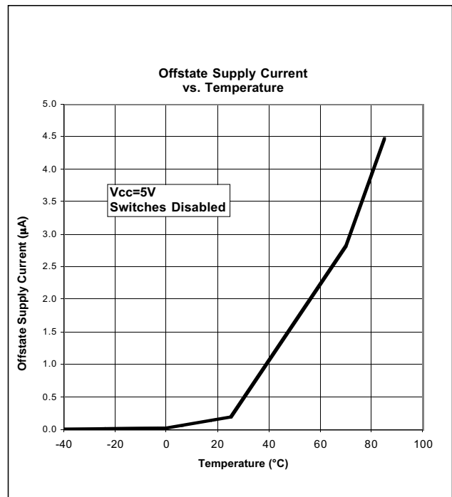
Figure 15. Off-state Supply Current vs. Temperature
