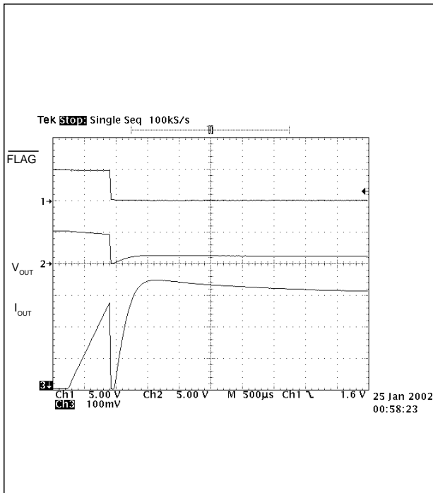
Figure 18. Current-Limit Response With a Ramped Load
