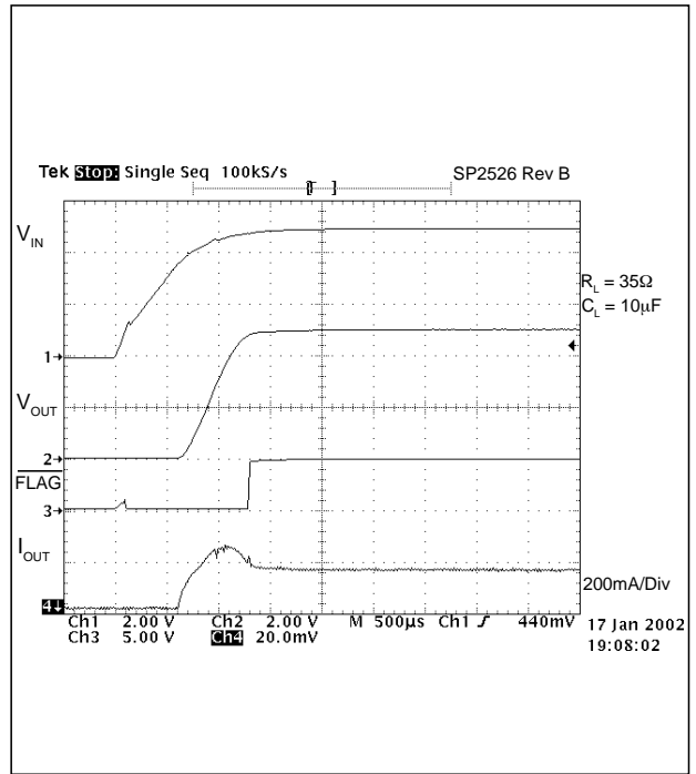
Figure 17. Input Voltage Response
