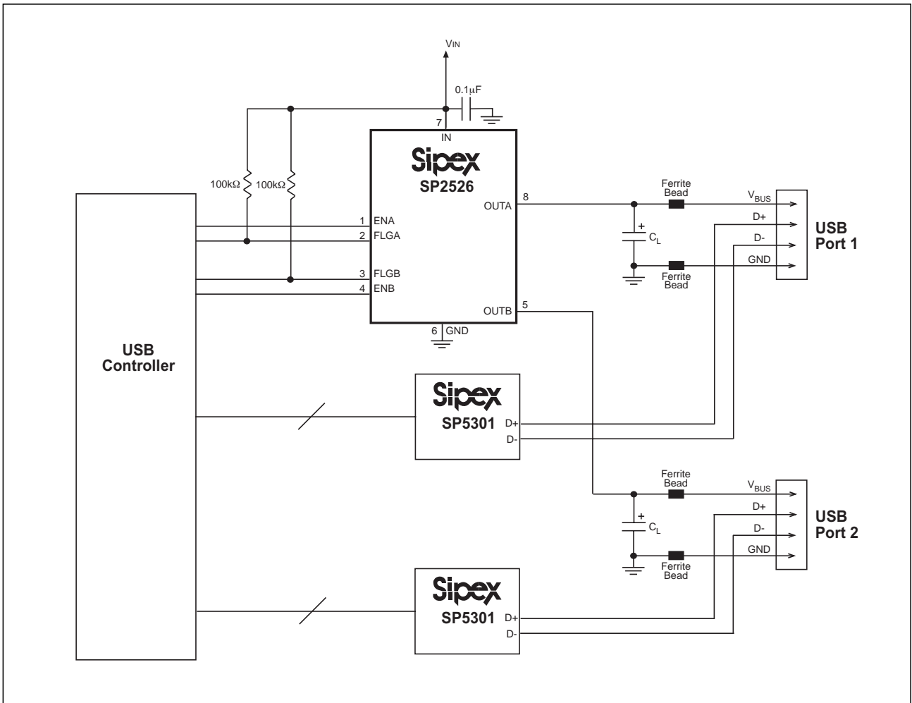
Figure 3. Typical Application Circuit for the SP2526
