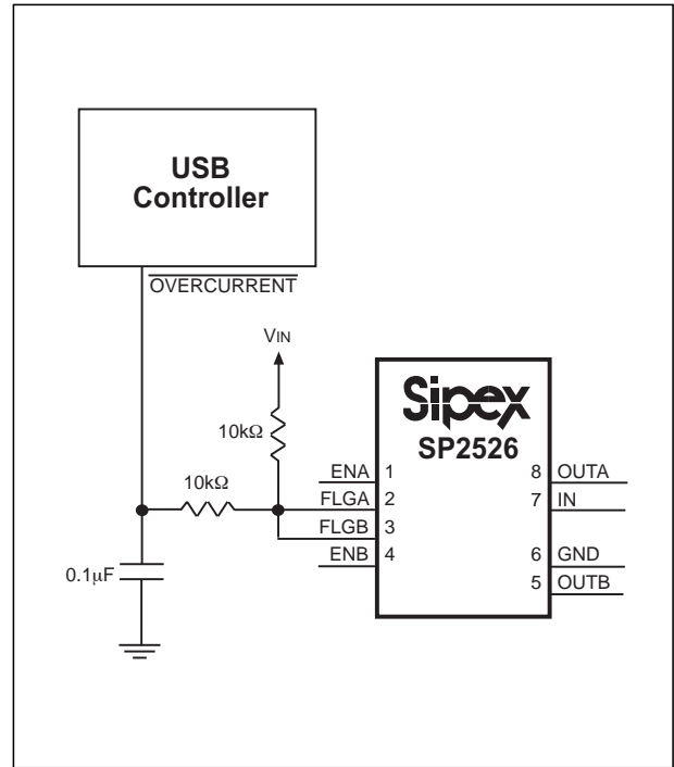
Figure 5. An RC Filter for Overcurrent Faults
