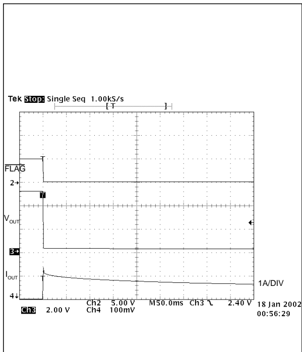
Figure 22. Short Circuit Response (Short Applied To Output)
