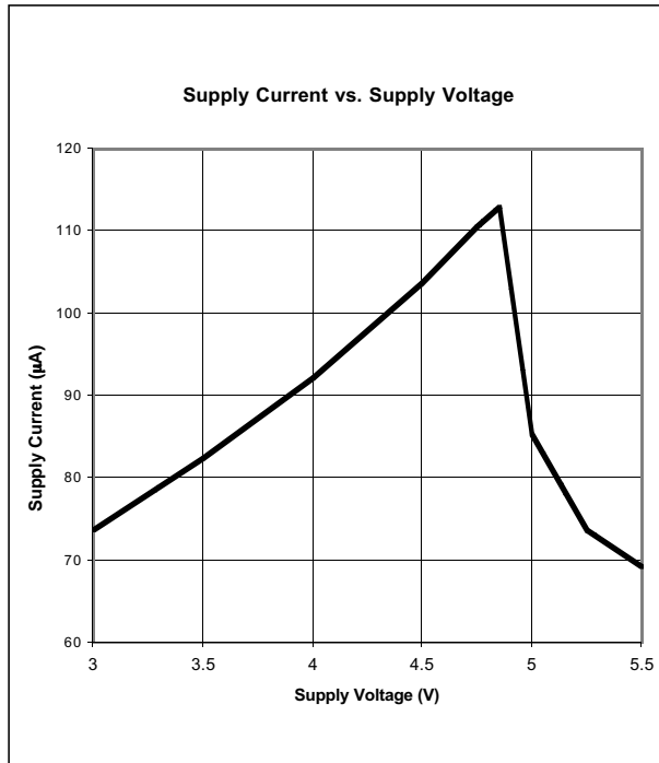
Figure 12. On-state Supply Current vs. Supply Voltage
