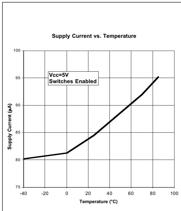
Figure 14. On-state Supply Current vs. Temperature
