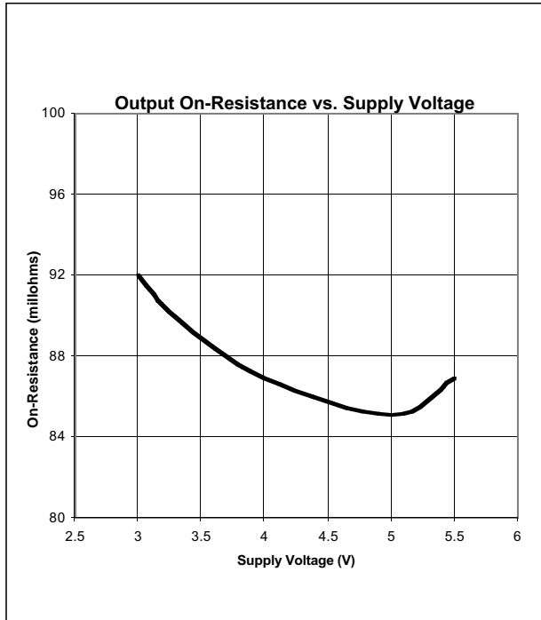
Figure 8. Output On-Resistance vs. Supply Voltage
