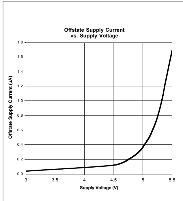
Figure 13. Off-state Supply Current vs. Supply Voltage
