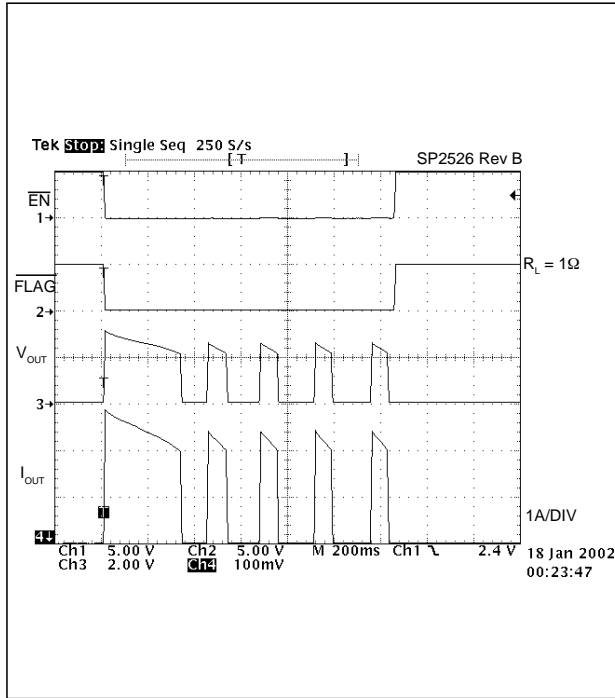
Figure 24. Short Circuit Response (Enable into Short Circuit)
