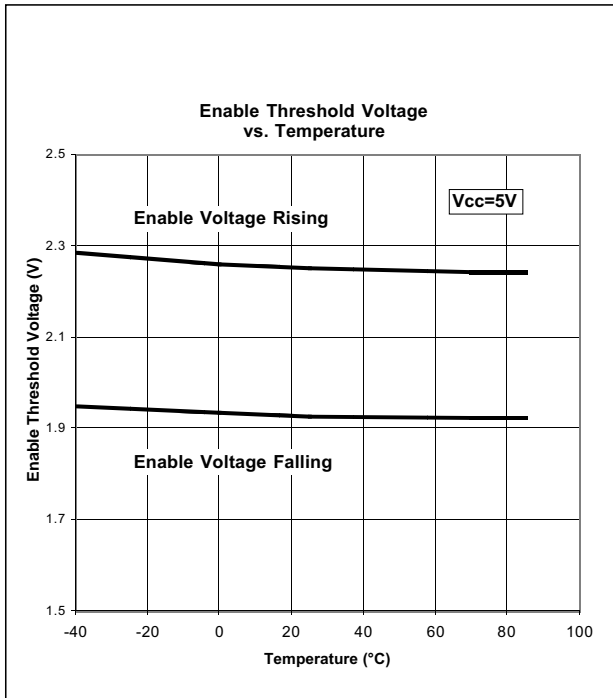
Figure 16. Control Threshold vs. Temperature
