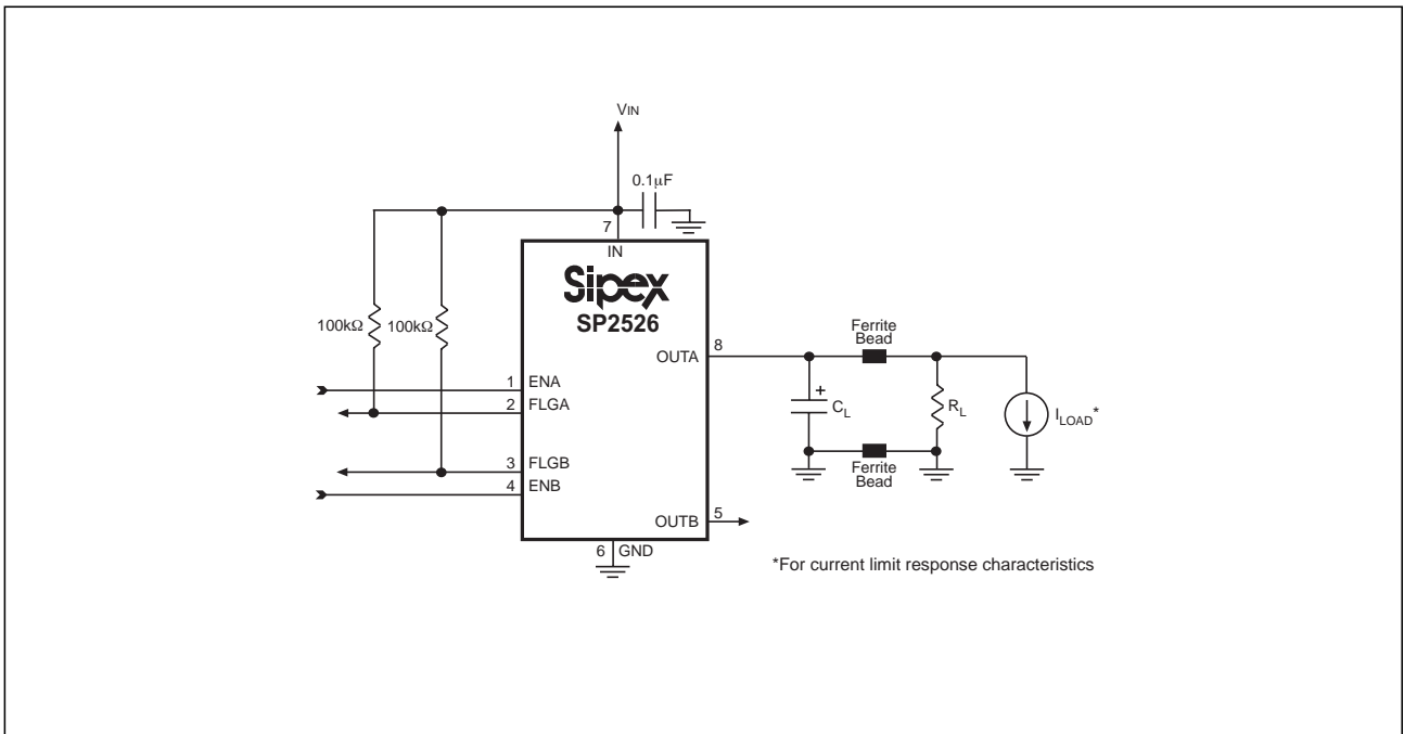
Figure 2. Test Circuit for the SP2526
