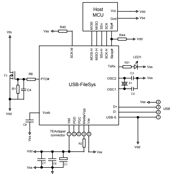
Figure 4. Typical Application Circuit, Internal Memory
