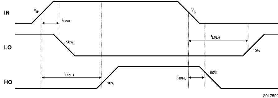
FIGURE 3. LM5106 Switching Time Definitions: t_{LPLH} , t_{LPHL} , t_{HPHL} , t_{HPLH}
