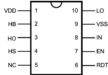
20175901 10-Lead MSOP or LLP See NS Number MUB10A, SDC10A
