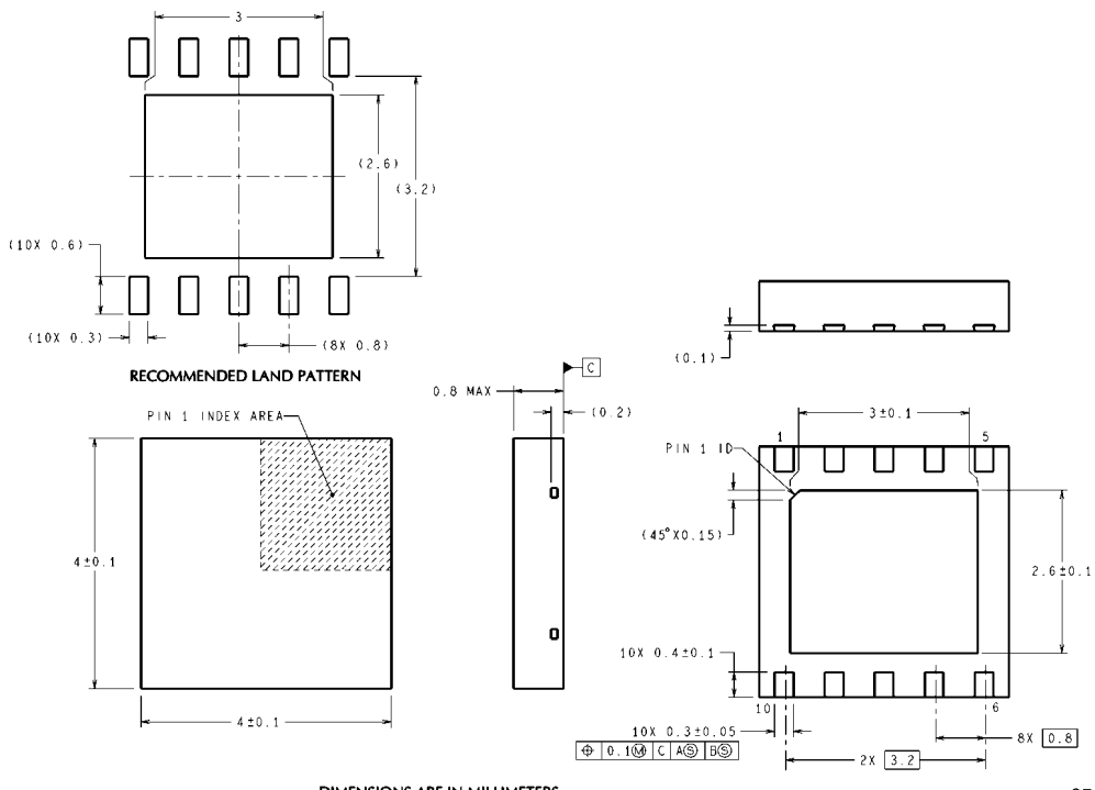
DIMENSIONS ARE IN MILLIMETERS LLP-10 Outline Drawing NS Package Number SDC10A
