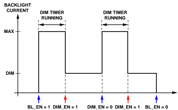
Figure 33. Dim Timer
