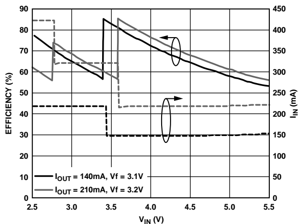
Figure 19. Typical Efficiency (Low Vf Diode)
