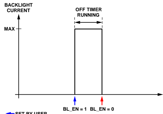
Figure 34. Off Timer
