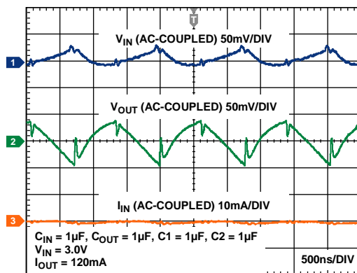
Figure 21. Typical Operating Waveforms, G = 1\times
