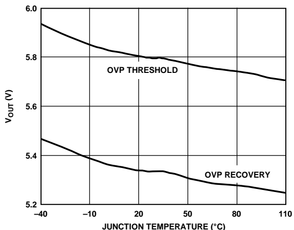
Figure 18. Typical Overvoltage Protection (OVP) Threshold
