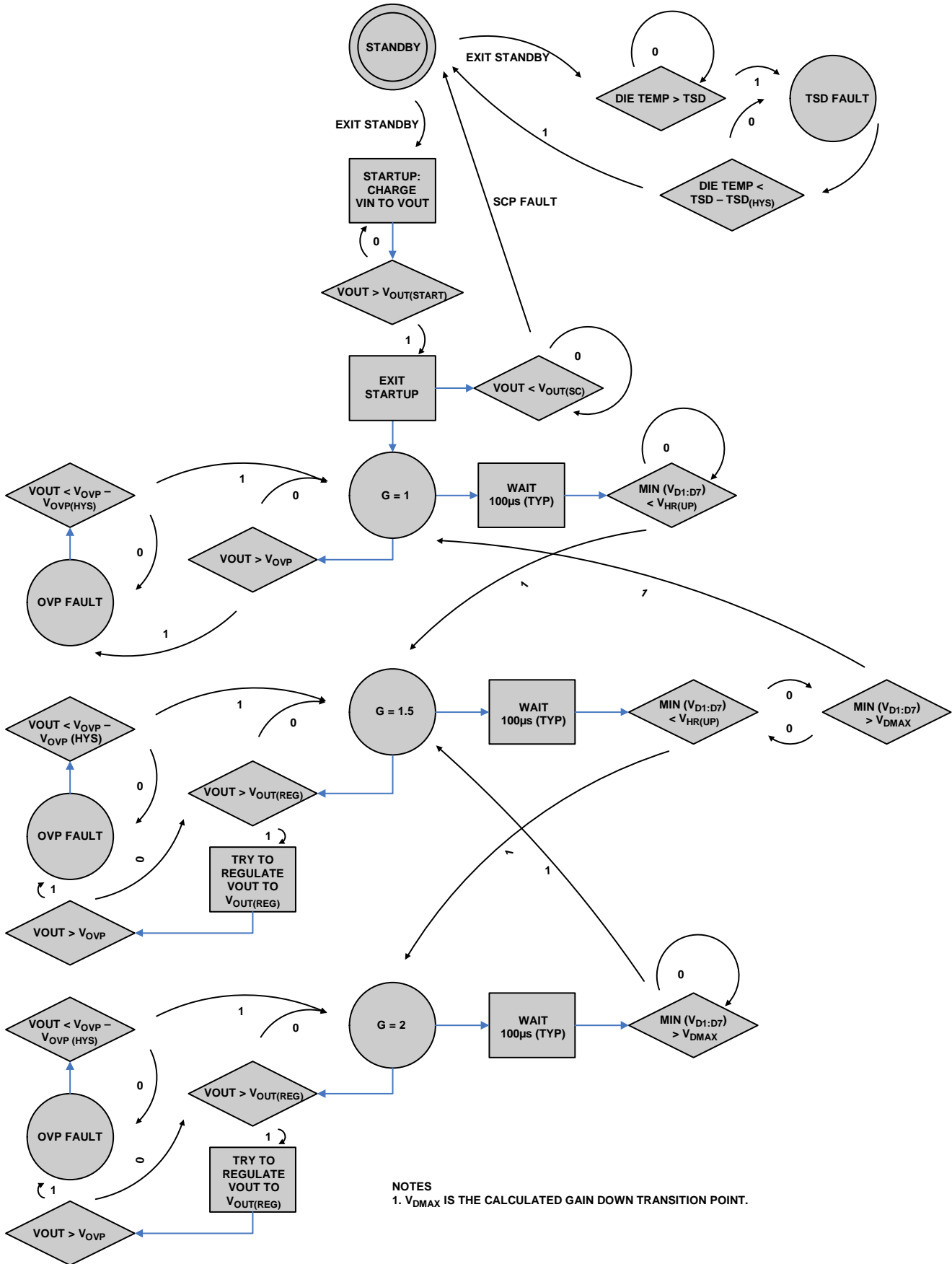
Figure 38. Fault State Machine Rev. A | Page 18 of 40
