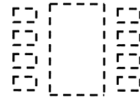
FIGURE 4. LLP Thermal Land Pad and Pin Pads
