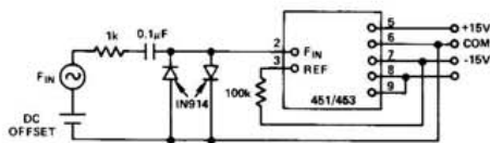
Figure 10. Input Diode Protection for High Voltage Transients
