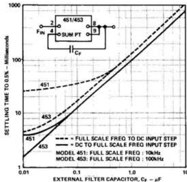
Figure 14. Settling Time Versus External Filter Capacitor
