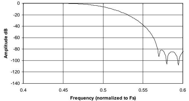
Figure 12. Double-speed Transition Band
