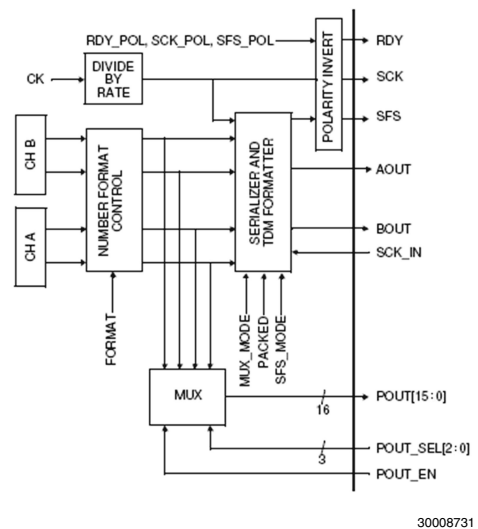
FIGURE 33. LM97593 output circuit
