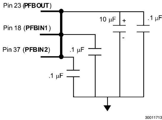
FIGURE 12. Power Feedback Connection
