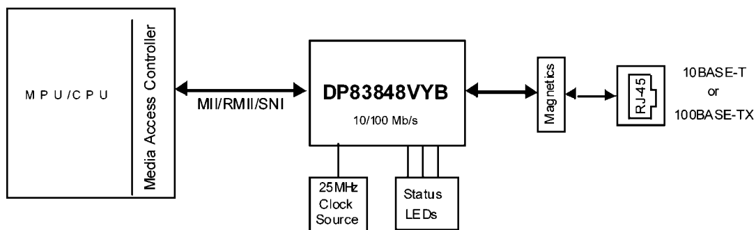
Typical Application
