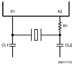
FIGURE 11. Crystal Oscillator Circuit
