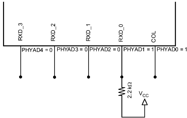
FIGURE 1. PHYAD Strapping Example
