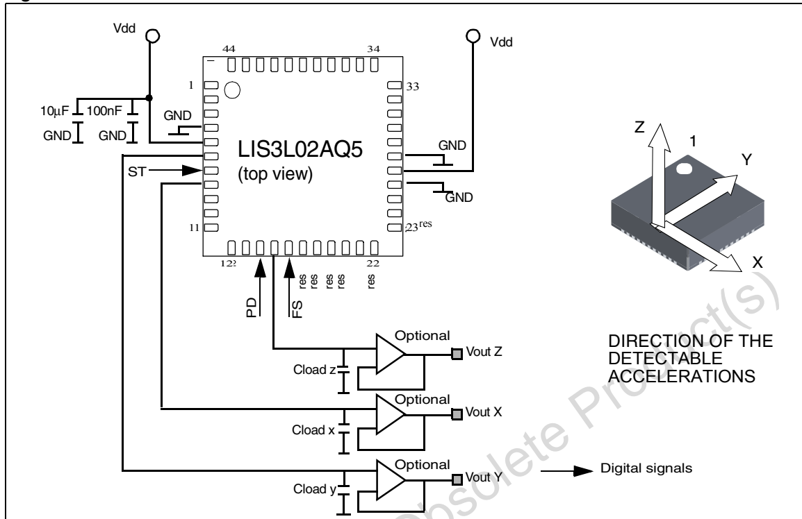
Figure 3. LIS3L02AQ5 Electrical Connection
