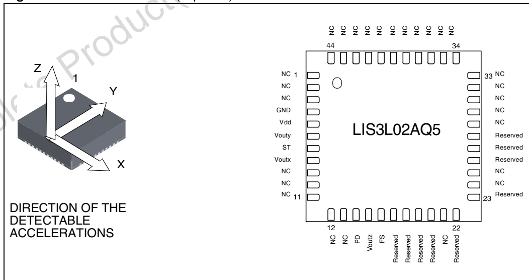
Figure 2. Pins Connection (Top view)
