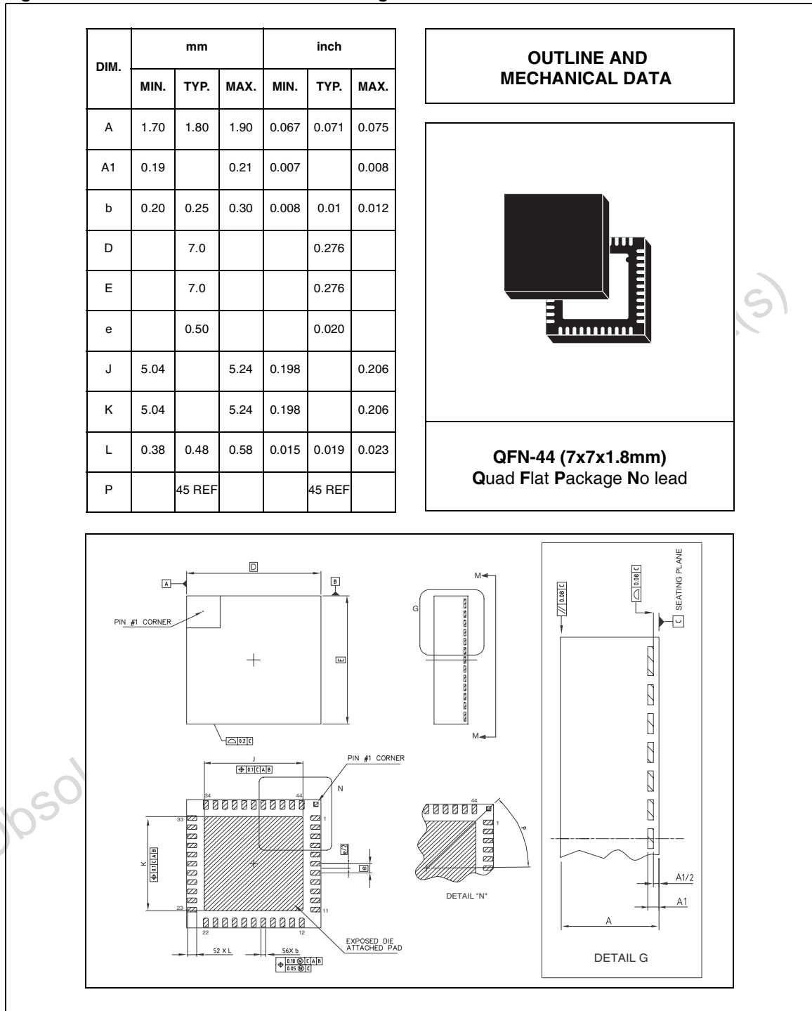
Figure 4. QFN-44 Mechanical Data & Package Dimensions
