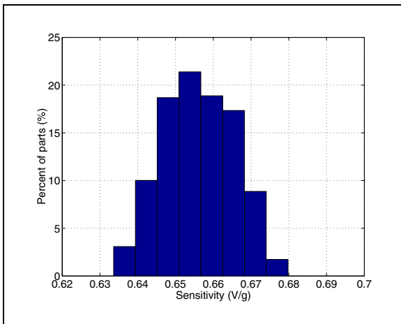
Figure 7. x-axis sensitivity at 3.3V
