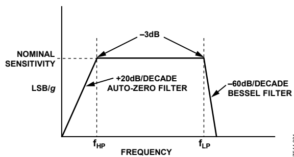
Figure 31. Bode Plot of ADXL180 Transfer Function
