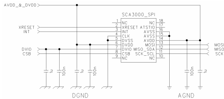
Figure 6 Application schematic
