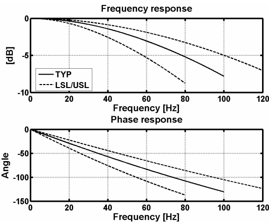
Figure 3 Frequency response of SCA3000-E05 in measurement mode
