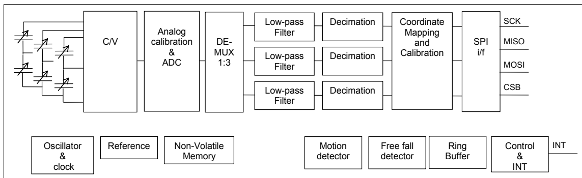
Figure 1 SCA3000-E05 Block Diagram
