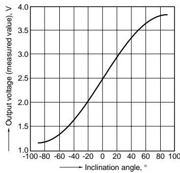
2. Inclination angle - Output voltage characteristics
