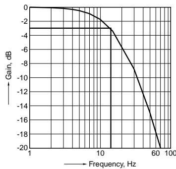
5. Frequency characteristics
