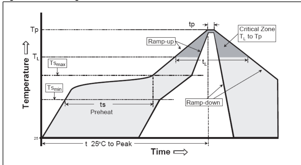
Figure 8. Soldering
