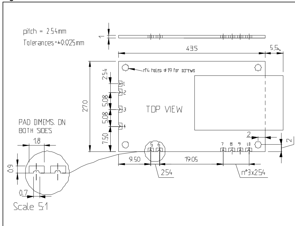
Figure 10. Mechanical dimensions
