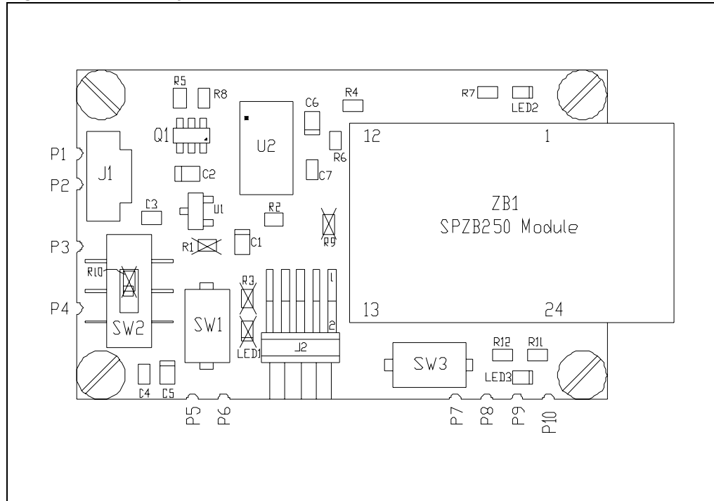
Figure 7. Board layout
