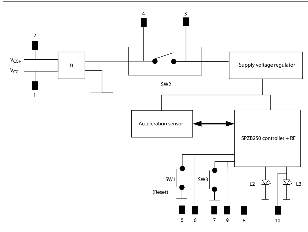
Figure 2. Block diagram
