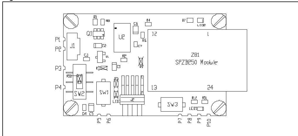
Figure 1. Connections
