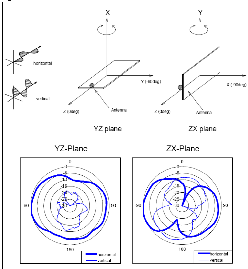
Figure 9. Measurement direction
