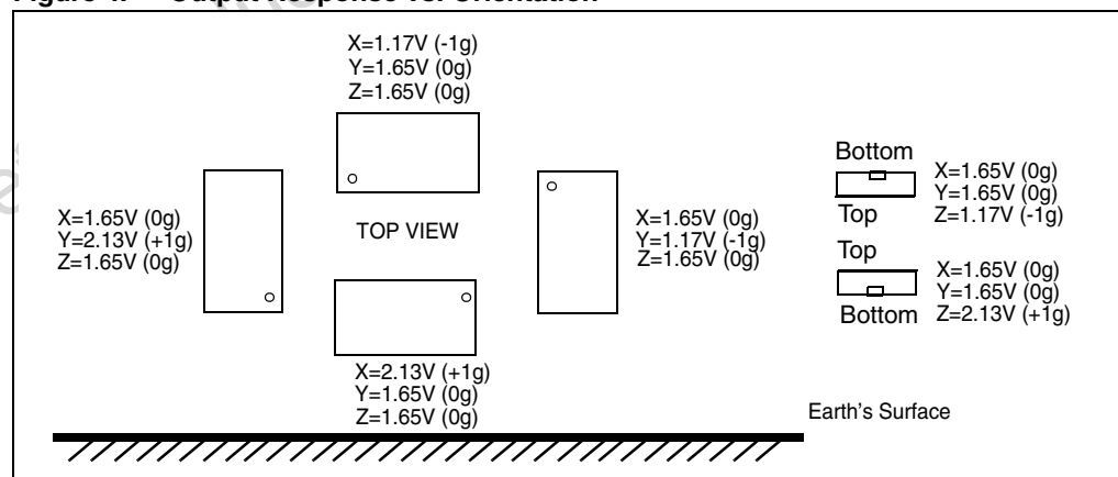
Figure 4 refers to LIS302ALB powered at 3.3V.
