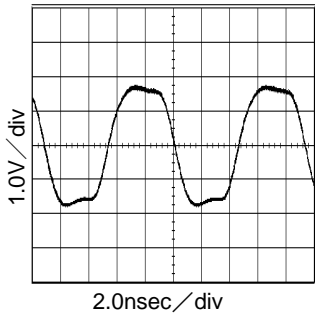
Fig.7 108MHz output wave At VDD=3.3V and CL=15pF
