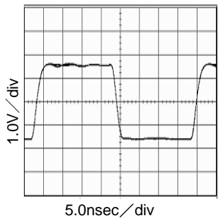
Fig.50 24MHz output waveform At VDD=3.3V and CL=15pF
