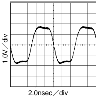
Fig.10 98MHz output wave At VDD=3.3V and CL=15pF
