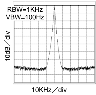
Fig.49 30MHz Spectrum At VDD=3.3V and CL=15pF
