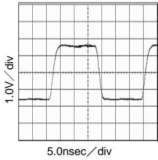
Fig.47 30MHz output waveform At VDD=3.3V and CL=15pF
