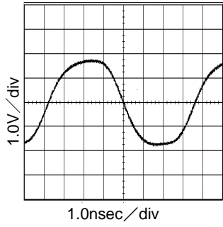
Fig.1 135MHz output wave At VDD=3.3V and CL=15pF
