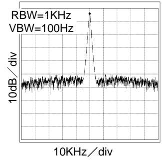
Fig.18 17.7MHz Spectrum At VDD=3.3V and CL=15pF
