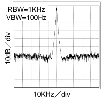
Fig.15 48MHz Spectrum At VDD=3.3V and CL=15pF
