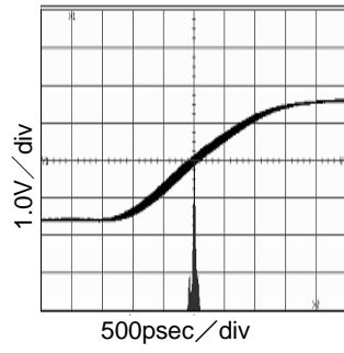
Fig.54 27MHz Period-Jitter At VDD=3.3V and CL=15pF
