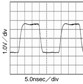
Fig.44 36MHz output waveform At VDD=3.3V and CL=15pF
