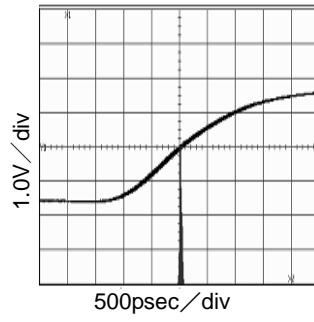
Fig.45 136MHz Period-Jitter At VDD=3.3V and CL=15pF
