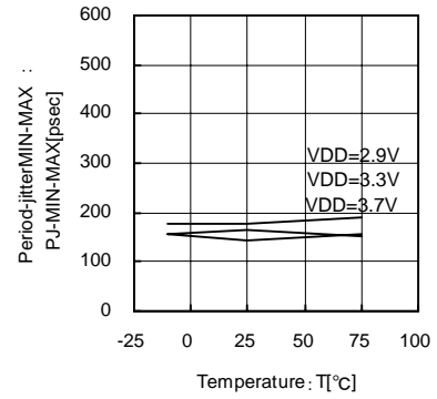
Fig.61 36MHz Temperature - Period-Jitter MIN-MAX
