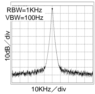
Fig.21 14.3MHz Spectrum At VDD=3.3V and CL=15pF
