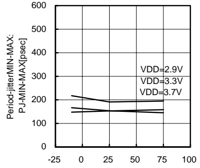
Fig.67 24MHz Temperature - Period-Jitter MIN-MAX
