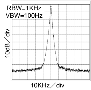
Fig.58 12MHz Spectrum At VDD=3.3V and CL=15pF
