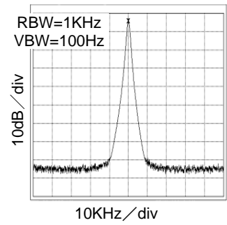
Fig.55 27MHz Spectrum At VDD=3.3V and CL=15pF
