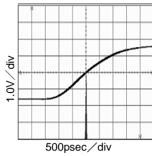
Fig.51 24MHz Period-Jitter At VDD=3.3V and CL=15pF
