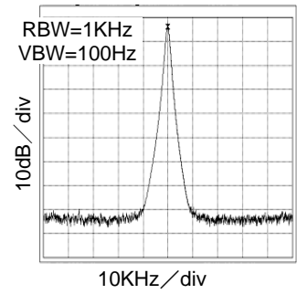
Fig.46 36MHz Spectrum At VDD=3.3V and CL=15pF
