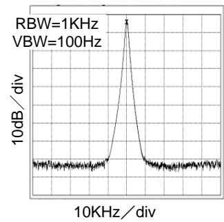
Fig.52 24MHz Spectrum At VDD=3.3V and CL=15pF
