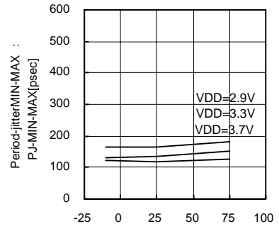
Fig.64 30MHz Temperature - Period-Jitter MIN-MAX
