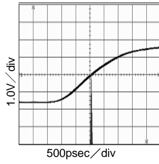
Fig.48 30MHz Period-Jitter At VDD=3.3V and CL=15pF
