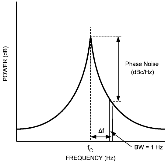
FIGURE 4. Phase Noise
