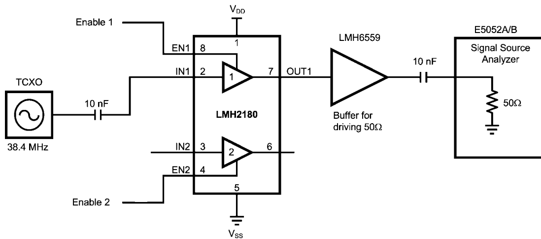
FIGURE 5. Measurement Setup
