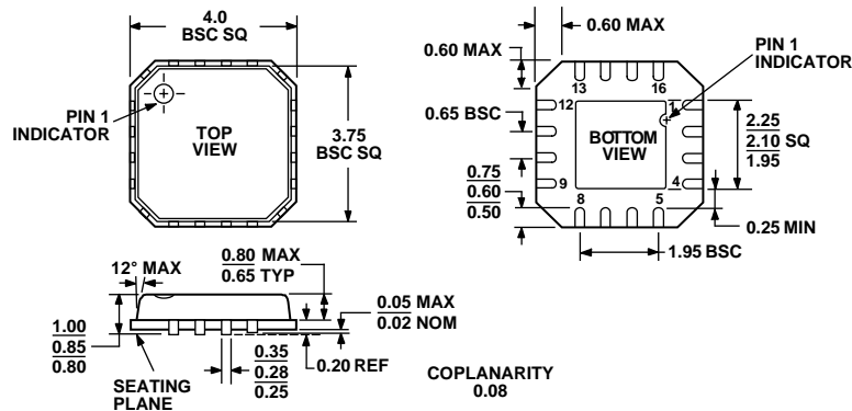
Figure 64. 16-Lead Lead Frame Chip Scale Package [LFCS] 4 mm x 4 mm Body (CP-16)
