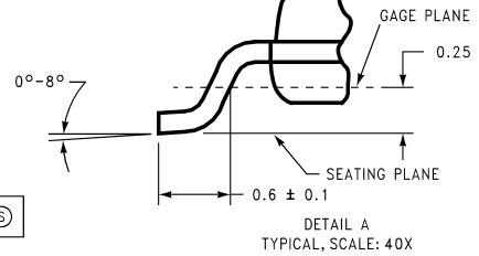
DETAIL A TYPICAL, SCALE: 40X
