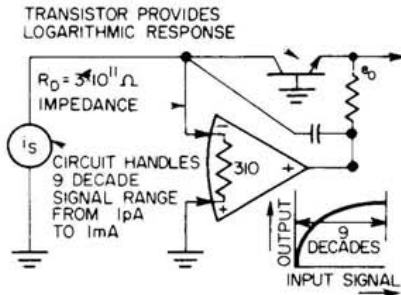
Nine Decade Logarithmic Amplifier
