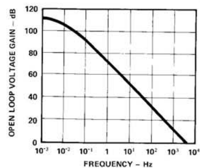
Frequency Response
