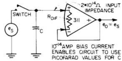
Low Capacitance Sample-and-Hold Amplifier
