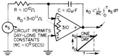
Long Term Integrator
