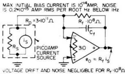
Ultra Sensitive Current Amplifier
