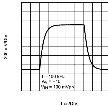
Large Signal Step Response with Gain = 10
