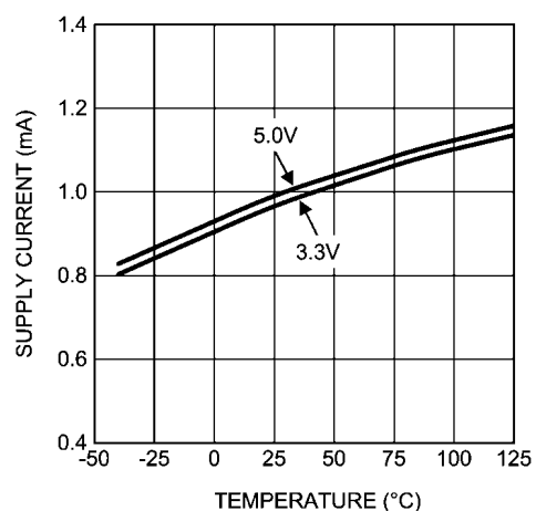
Supply Current vs. Temperature Quad LMV834
