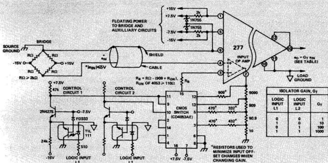
Figure 7. Programmable Gain Bridge Transducer Amplifier
