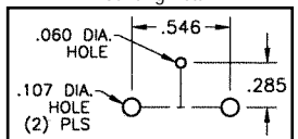
Mounting Detail
