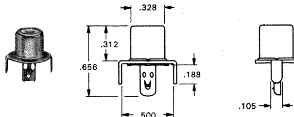
Mounting Detail
