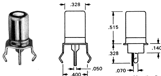
Mounting Detail
