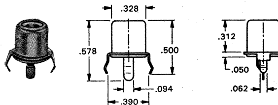
Mounting Detail
