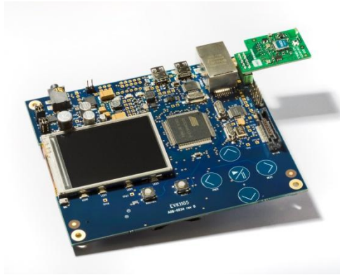
* Photo of the SPB105 connected with the SPI-card interface on the EVK1105. Ready-made downloadable reference designs can be started within minutes and development can start at once.
