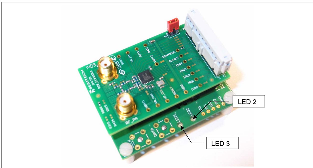
Figure 2: SM1231 Module Mounted on USB Bridge
