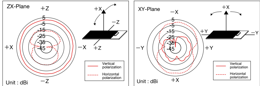
Typical characteristics of radiation pattern (@2.45GHz)
