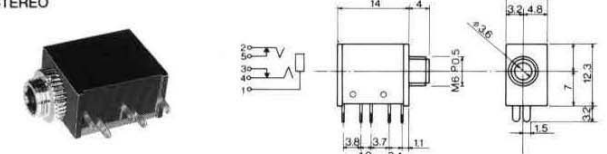
No.MJ-352W-C (φ 3.5) STEREO
