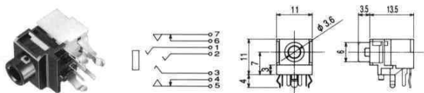
No.M03-610 (φ 3.5) STEREO
