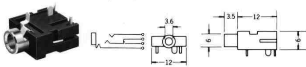
No.MJ-158L PANEL MOUNT 3-CON. STEREO MINIATURE JACK. (SINGLE CLOSED) Net Weight : 2 gr. (φ 3.5)
