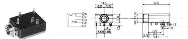
No.MJ-352W-C (φ 3.5) STEREO
