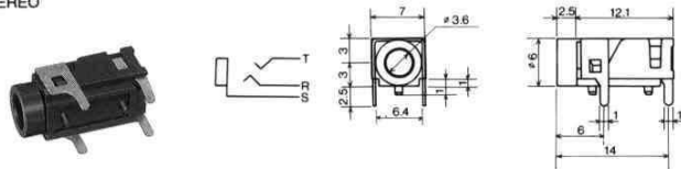
No.M03-610 (φ 3.5) STEREO
