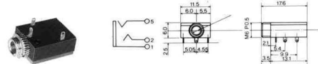
No.MJ-352W-0 (φ 3.5) STEREO
