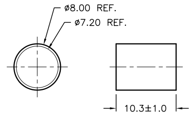
SLEEVE TUBE
