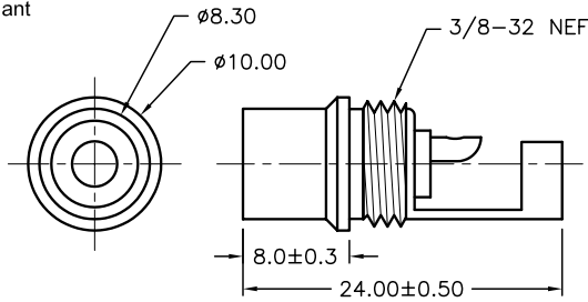
BODY
