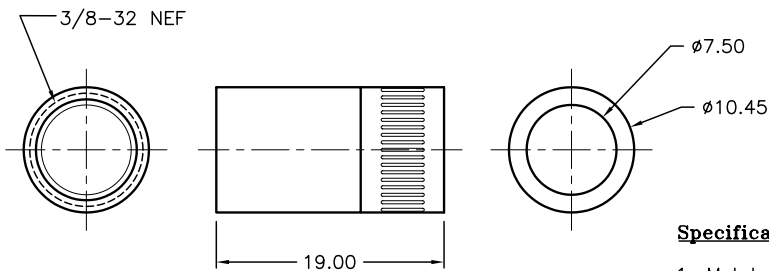
HANDLE
