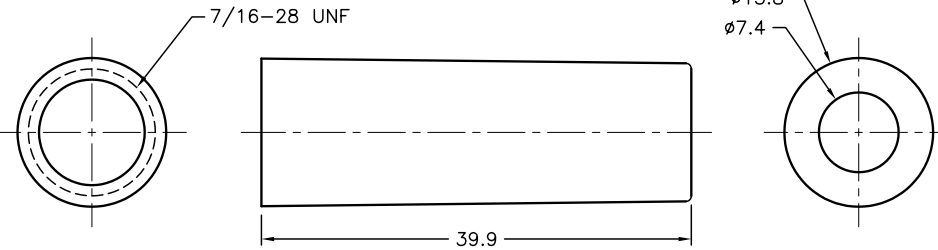
PLASTIC HANDLE
