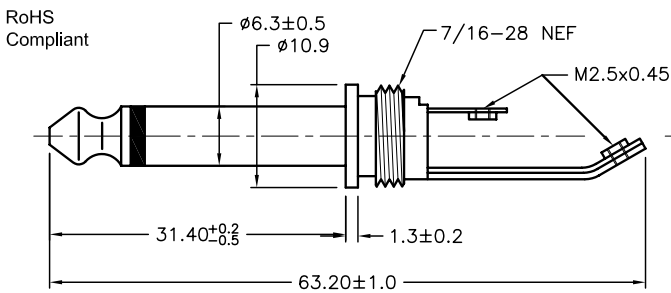
BODY
