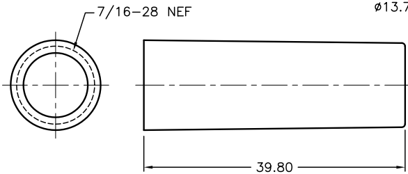
HANDLE
