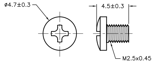
SCREW (2PCS)
