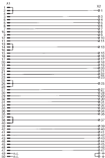
Wiring diagram
