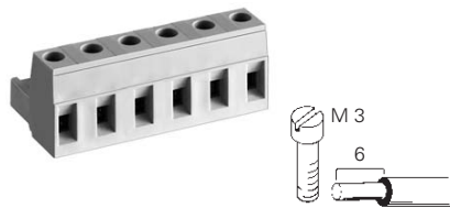
Type 8313 B/..., 8413 B/... plug-in 180° to wire entry
