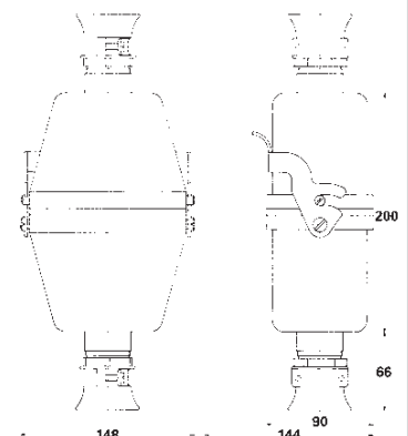
48pole connection
