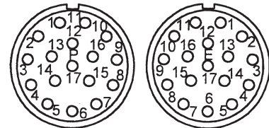
View from mating side
