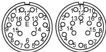
View from mating side
