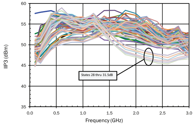
Input IP3 versus Frequency, All States, 25C
