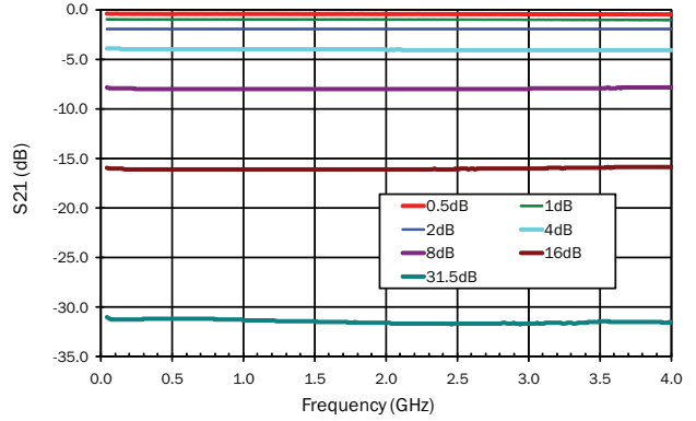
Normalized Attenuation, Major States
