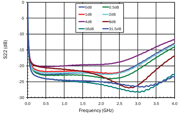
RF2 RL versus Frequency, Major States
