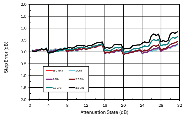
Step Error versus Attenuation (no ACG caps)
