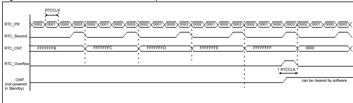
Figure 157. RTC Overflow waveform example with PR=0003
