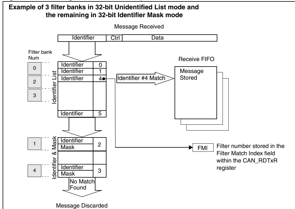
Figure 202. Filtering mechanism - example
