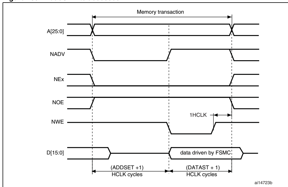
Figure 169. ModeC write accesses
