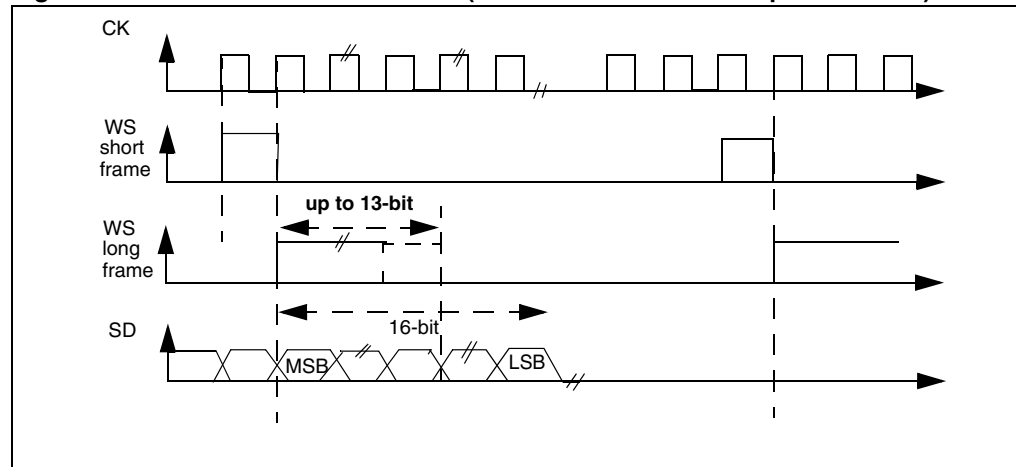
Figure 228. PCM standard waveforms (16-bit extended to 32-bit packet frame)
