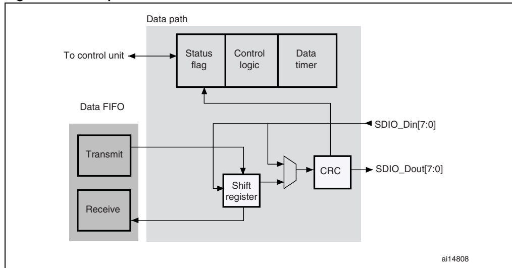
Figure 188. Data path
