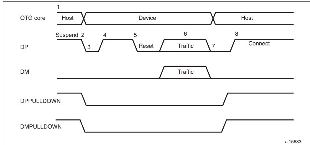
Figure 282. A-device HNP
