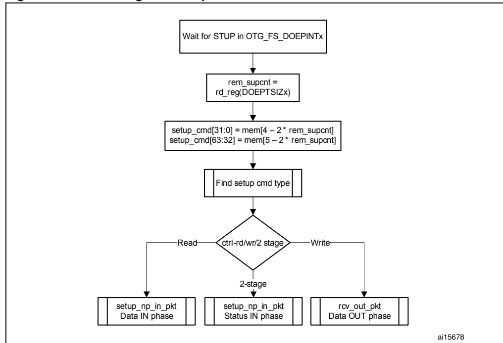
Figure 277. Processing a SETUP packet
