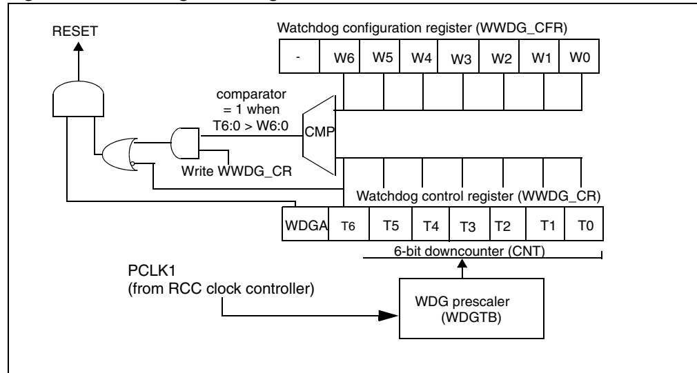
Figure 159. Watchdog block diagram
