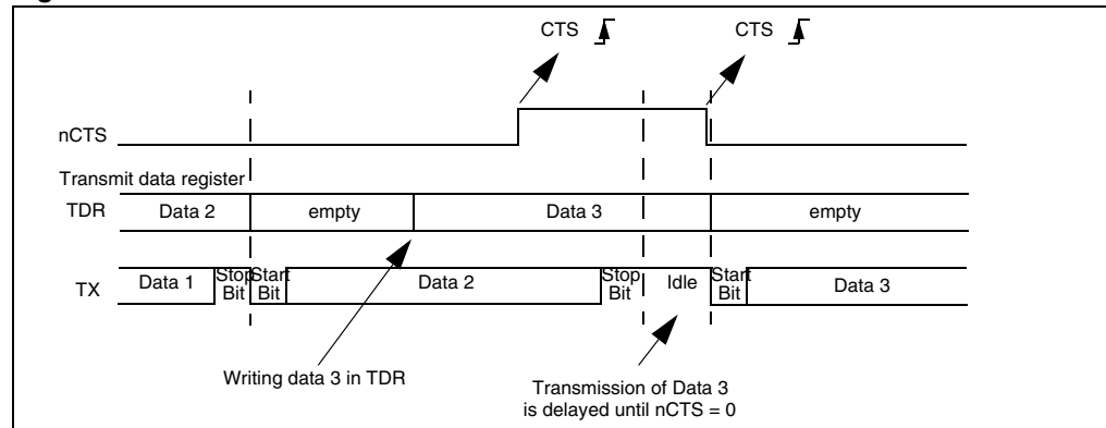
Figure 258. CTS flow control
