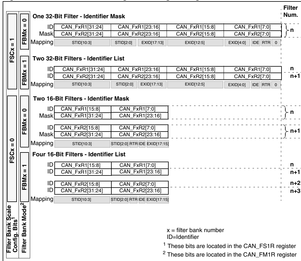
Figure 200. Filter bank scale configuration - register organization
