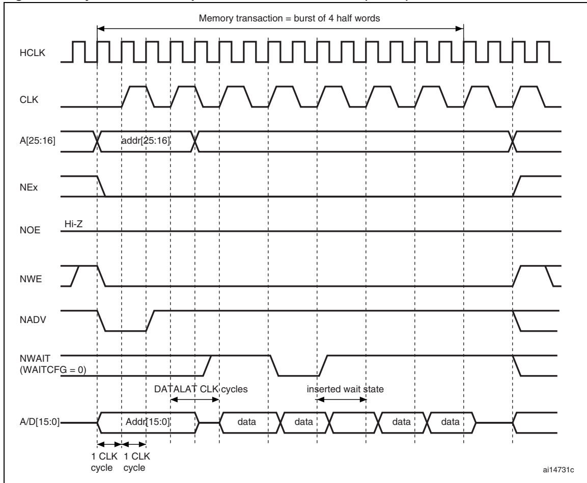
Figure 174. Synchronous multiplexed write mode - PSRAM (CRAM)
