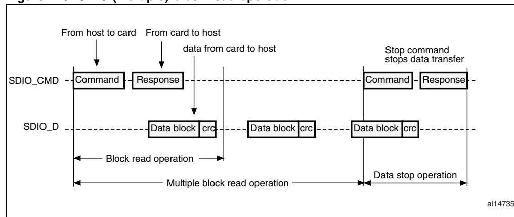
Figure 178. SDIO (multiple) block read operation
