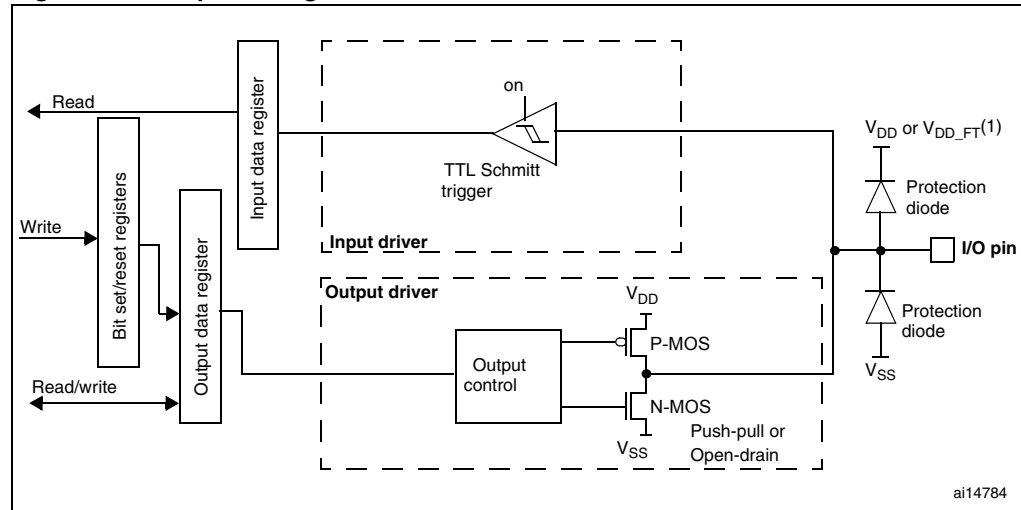
Figure 16. Output configuration
