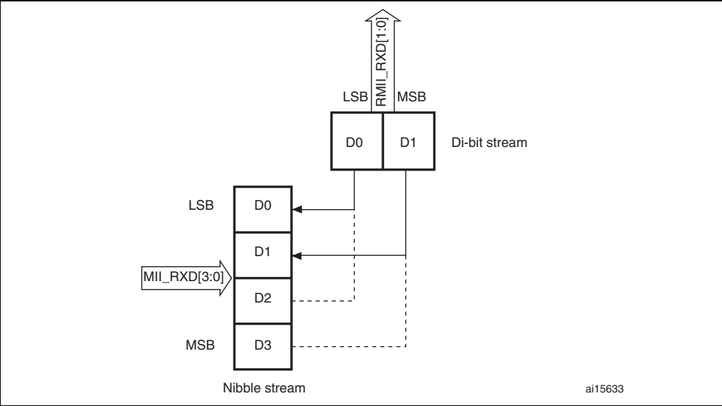
Figure 301. Reception with no error
