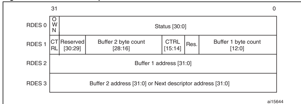
Figure 316. Rx DMA descriptor structure
