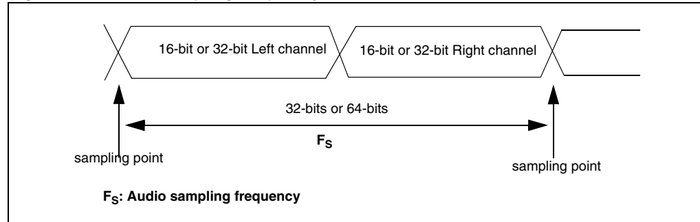
Figure 229. Audio sampling frequency definition
