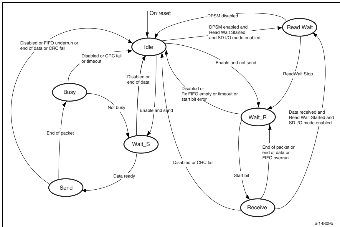
Figure 189. Data path state machine (DPSM)
