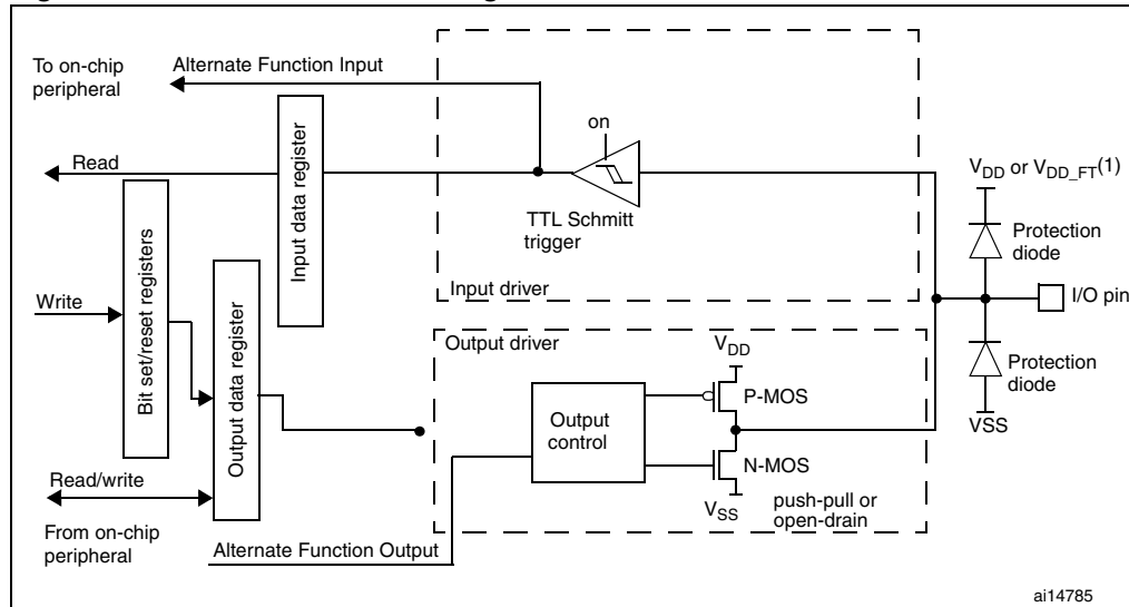
Figure 17. Alternate function configuration
