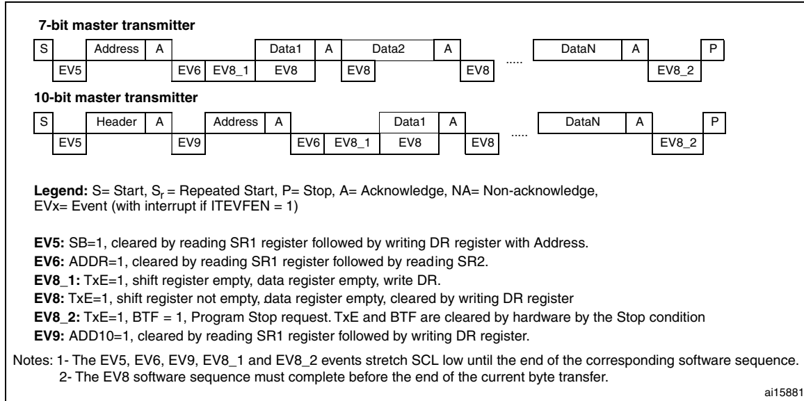
Figure 235. Transfer sequence diagram for master transmitter
