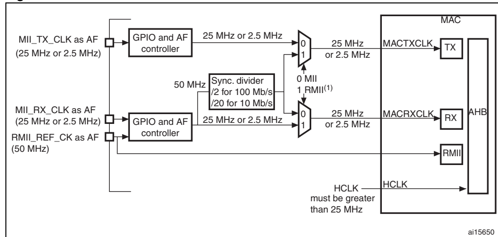
Figure 292. Clock scheme
