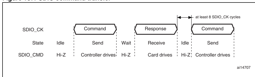
Figure 187. SDIO command transfer
