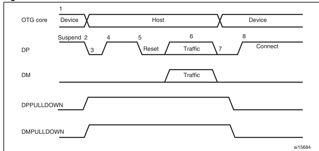
Figure 283. B-device HNP
