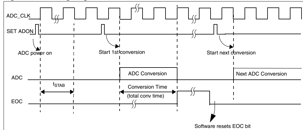
Figure 26. Timing diagram
