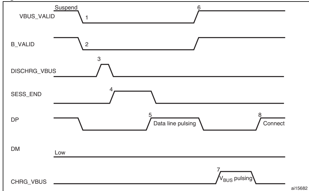
Figure 281. B-device SRP
