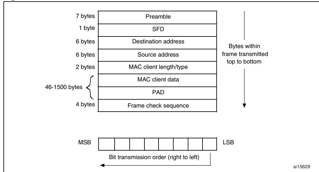
Figure 294. MAC frame format
