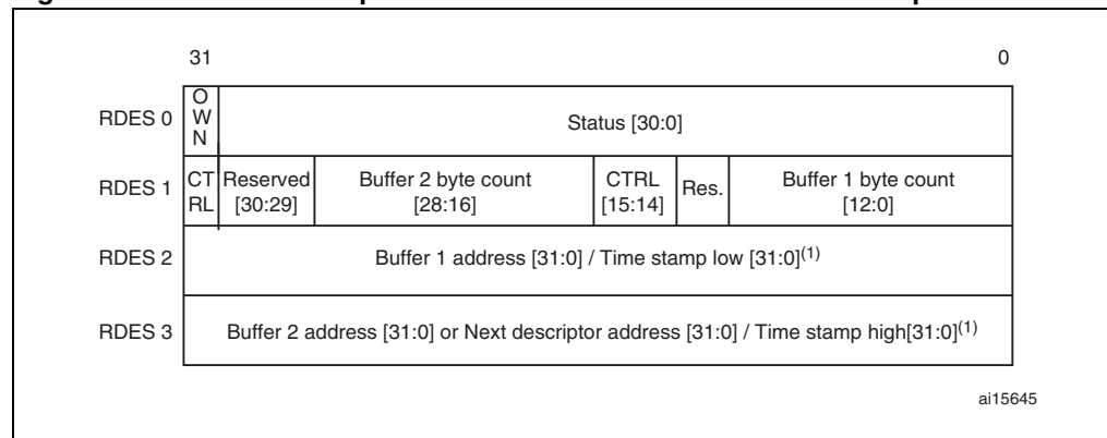
Figure 317. Receive descriptor fields format with IEEE1588 time stamp enabled
