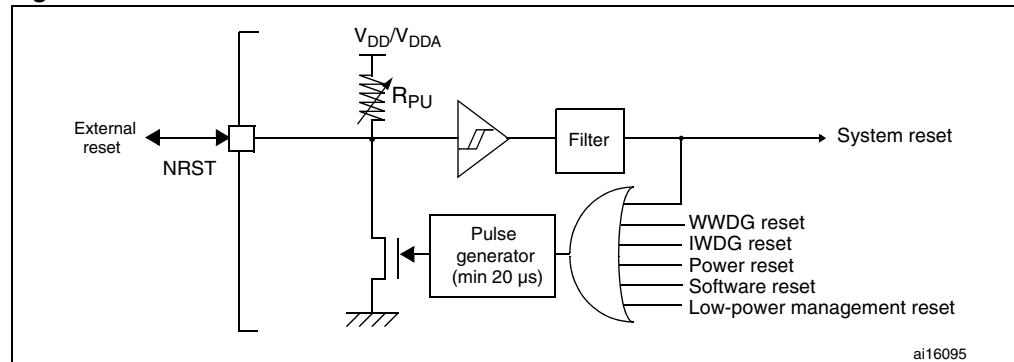
Figure 7. Reset circuit
