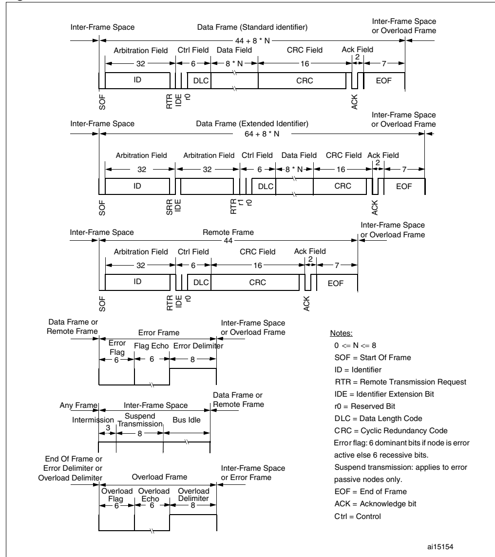
Figure 205. CAN frames
