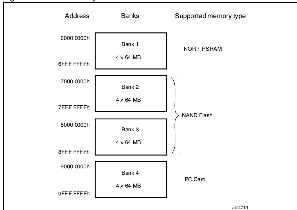
Figure 161. FSMC memory banks
