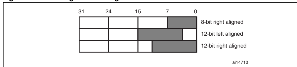
Figure 44. Data registers in single DAC channel mode
