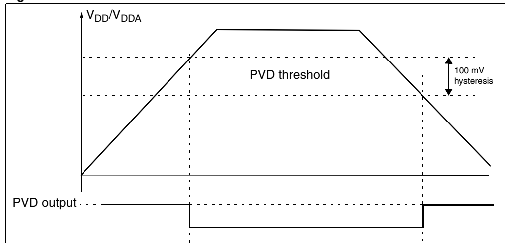
Figure 6. PVD thresholds
