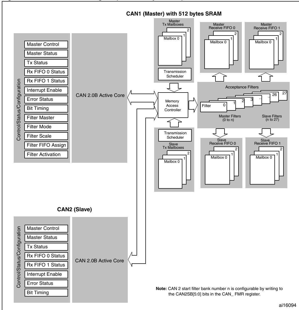
Figure 193. Dual CAN block diagram (connectivity devices)
