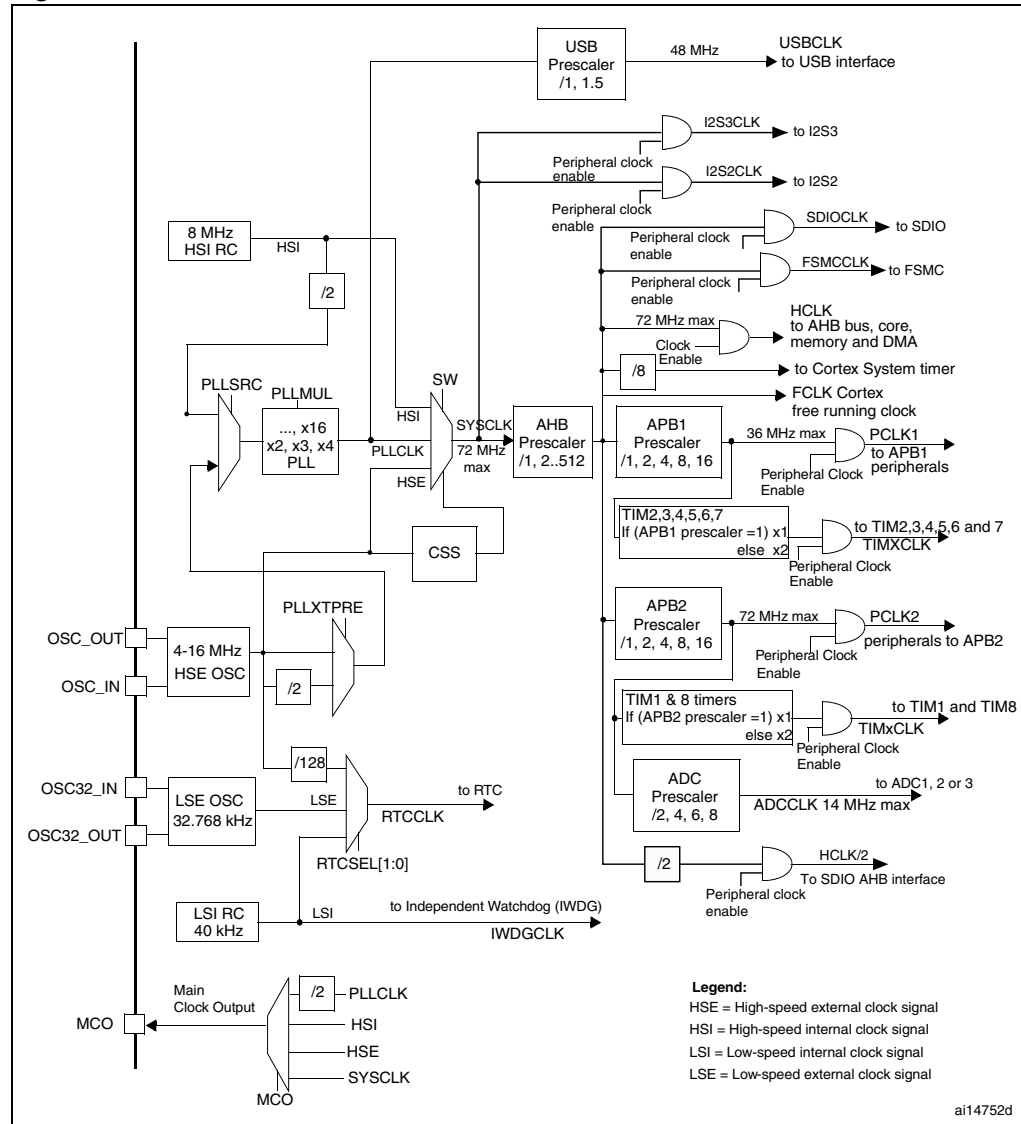
Figure 8. Clock tree
