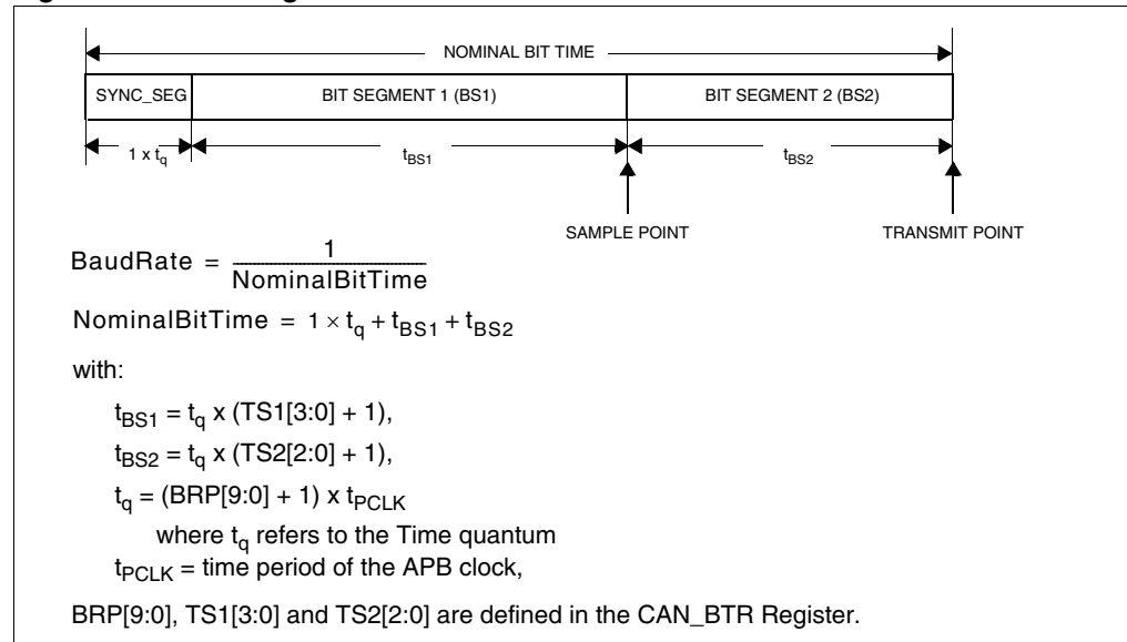
Figure 204. Bit timing
