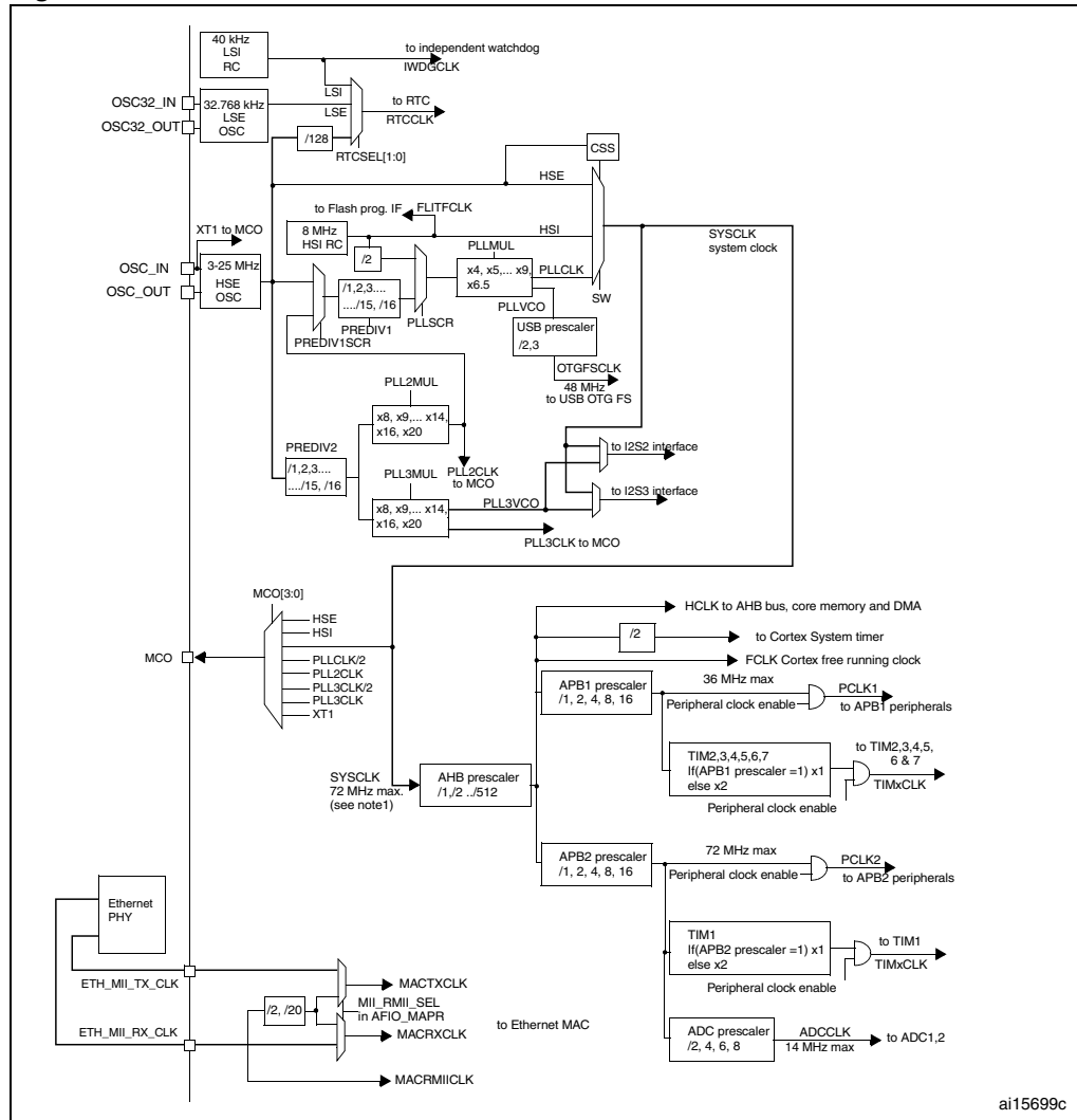
Figure 11. Clock tree
