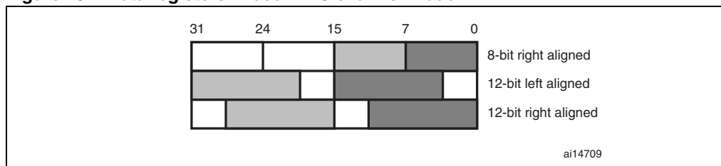
Figure 45. Data registers in dual DAC channel mode
