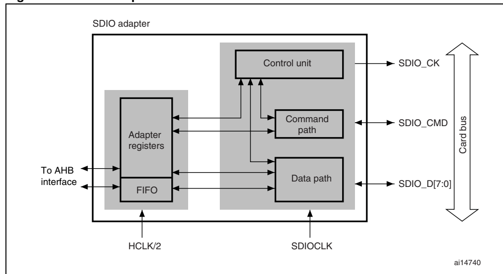
Figure 183. SDIO adapter
