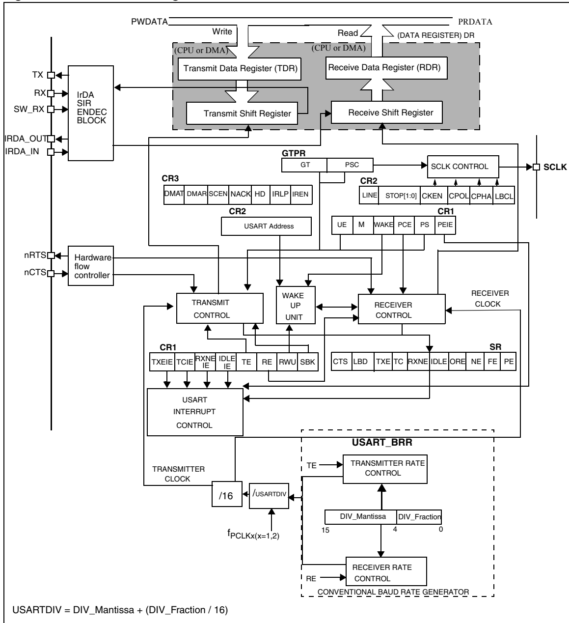
Figure 238. USART block diagram
