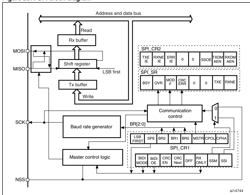
Figure 207. SPI block diagram
