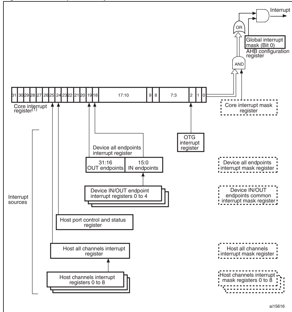
Figure 268. Interrupt hierarchy
