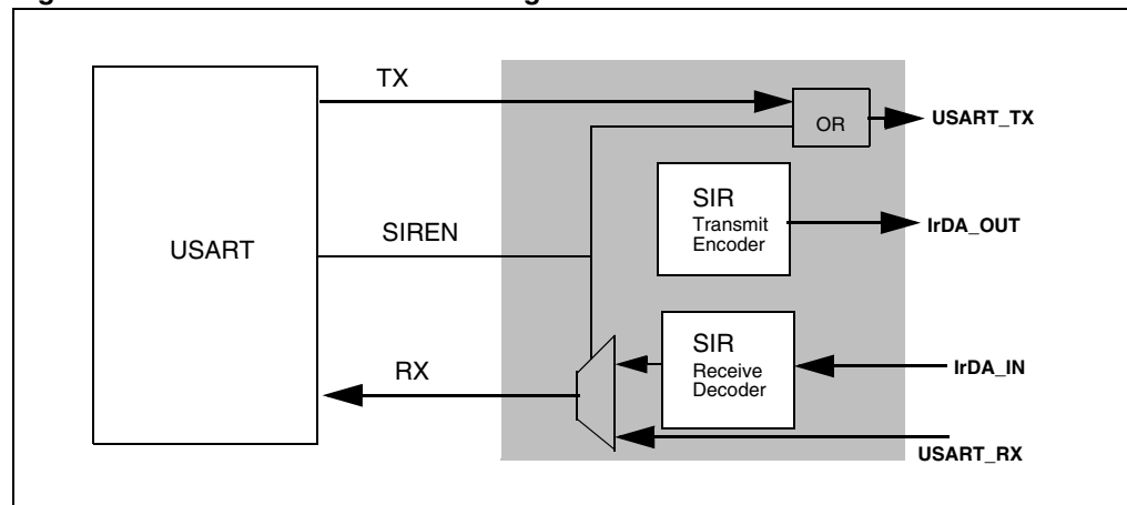
Figure 254. IrDA SIR ENDEC- block diagram
