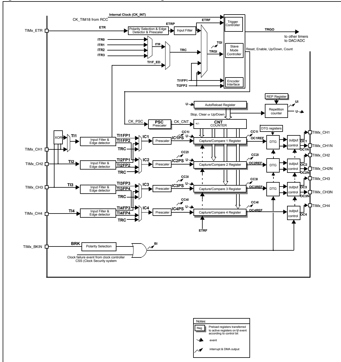
Figure 51. Advanced-control timer block diagram
