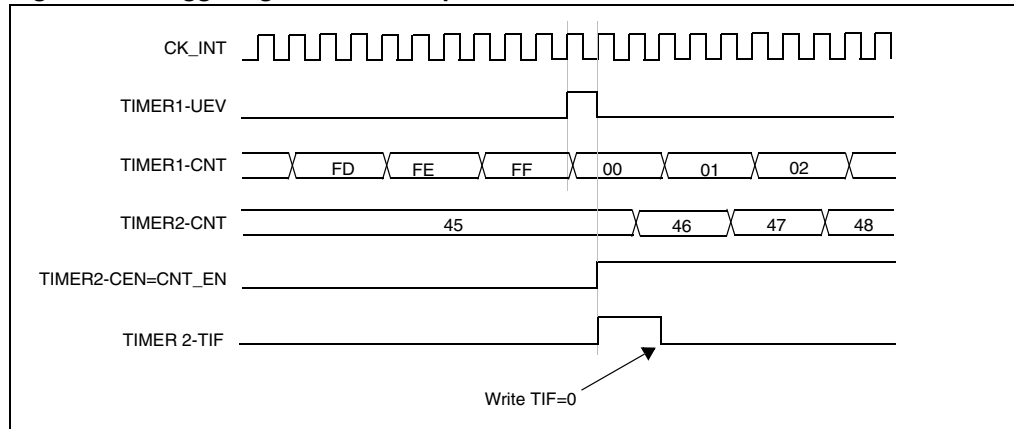
Figure 142. Triggering timer 2 with update of timer 1
