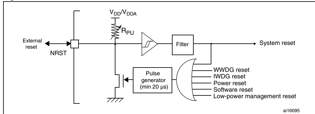
Figure 10. Reset circuit
