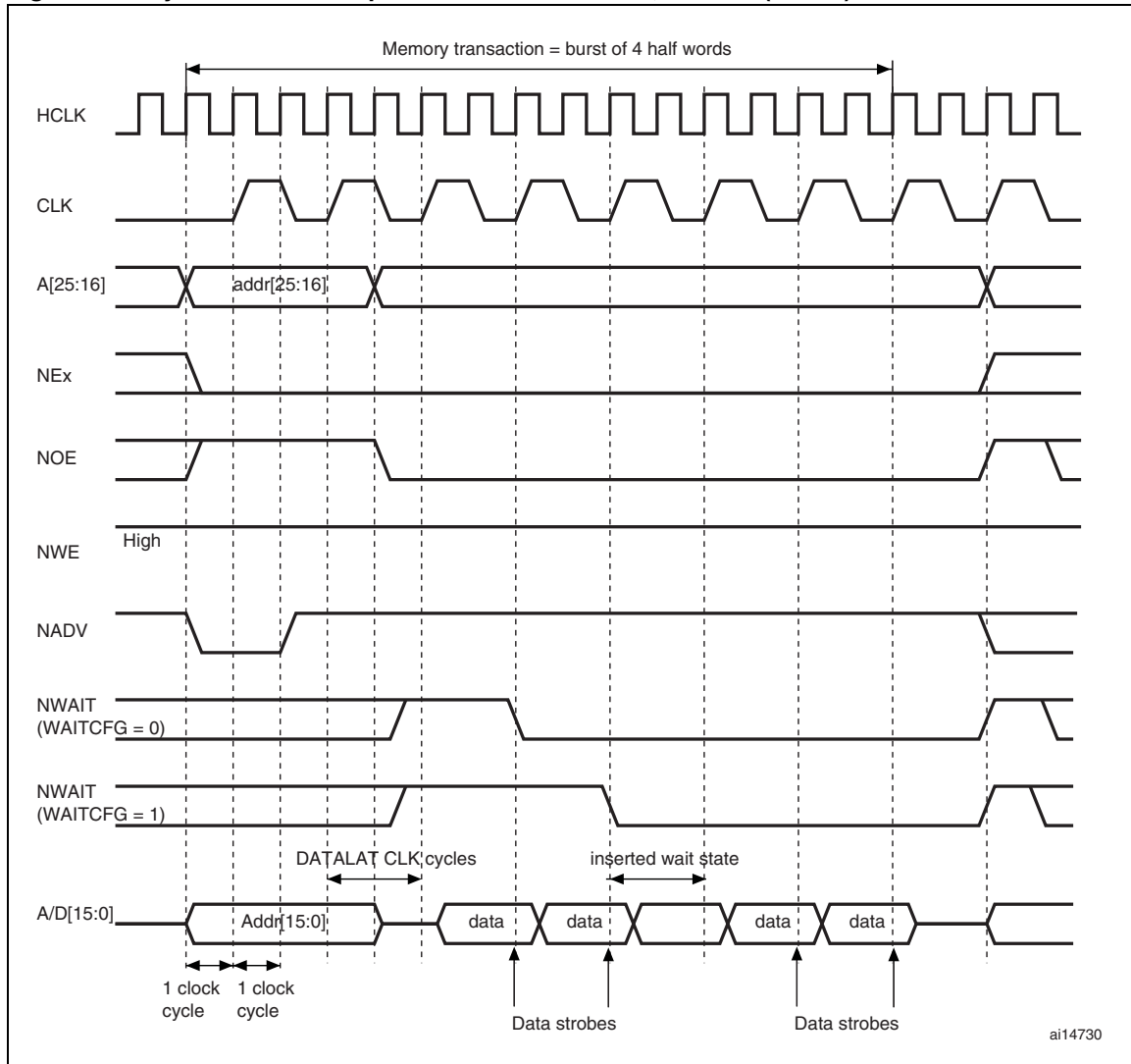
Figure 173. Synchronous multiplexed read mode - NOR, PSRAM (CRAM)
