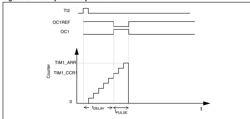
Figure 131. Example of one pulse mode.
