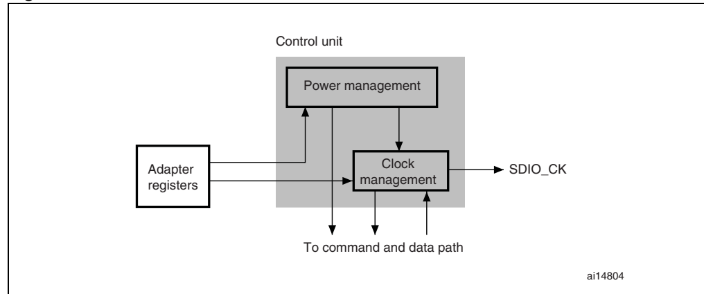
Figure 184. Control unit
