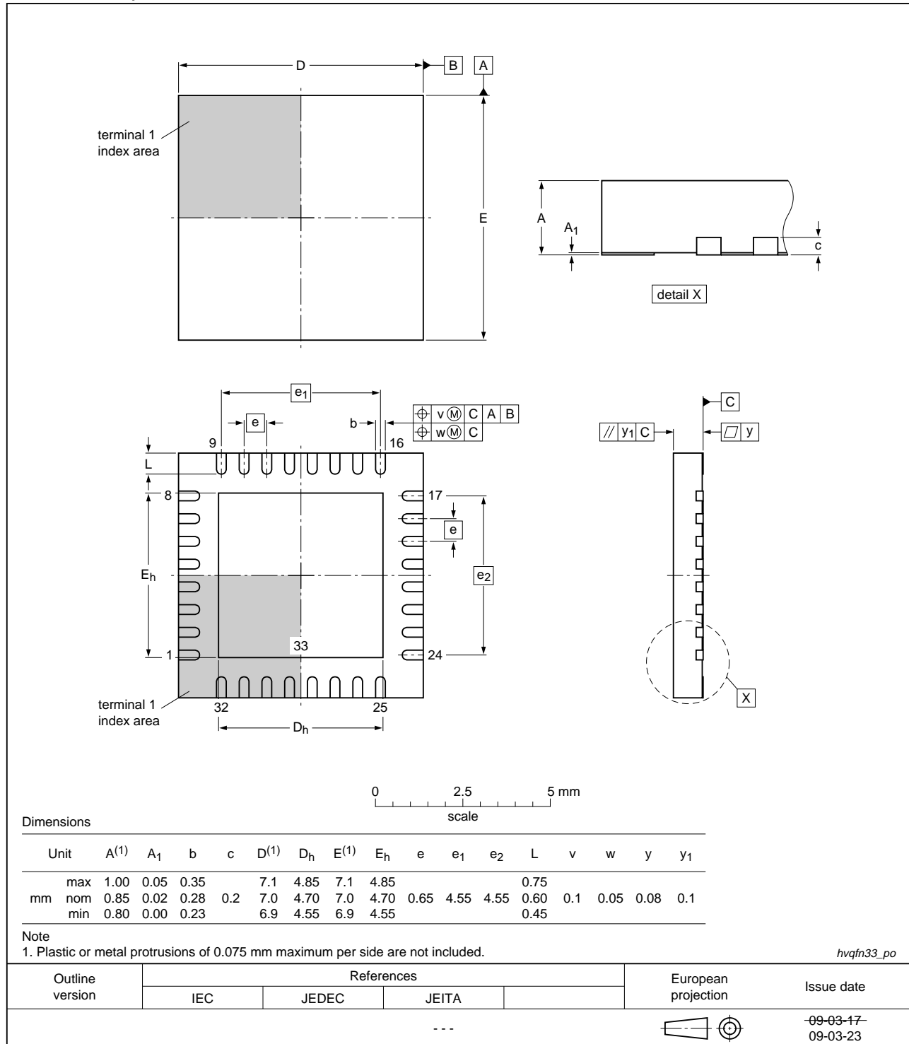
Fig 27. Package outline (HVQFN33)
