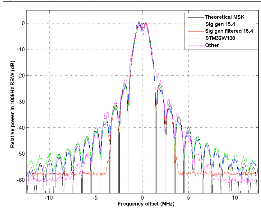
Figure 1. Comparison of spectra, 25 MHz span
